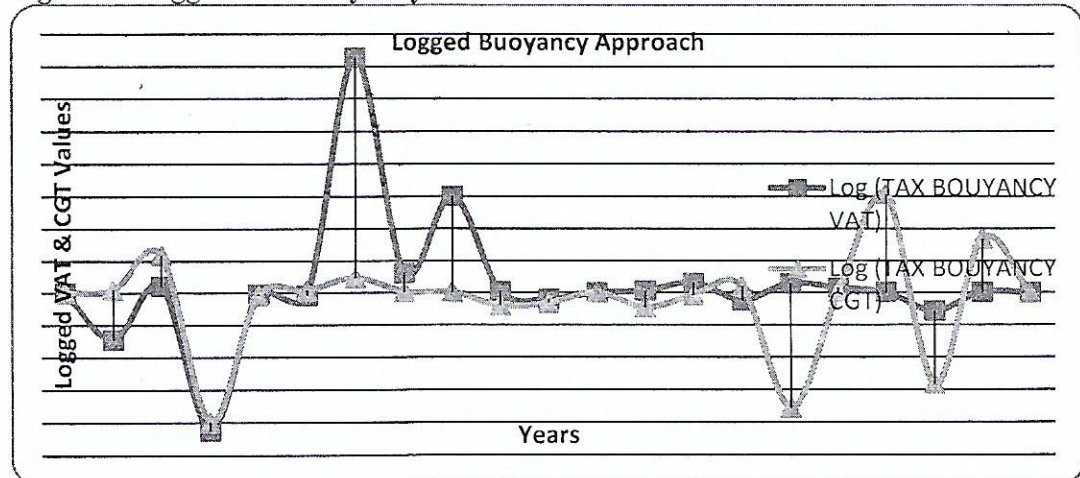
Figure 3: Logged Tax Buoyancy of VAT and CGT
