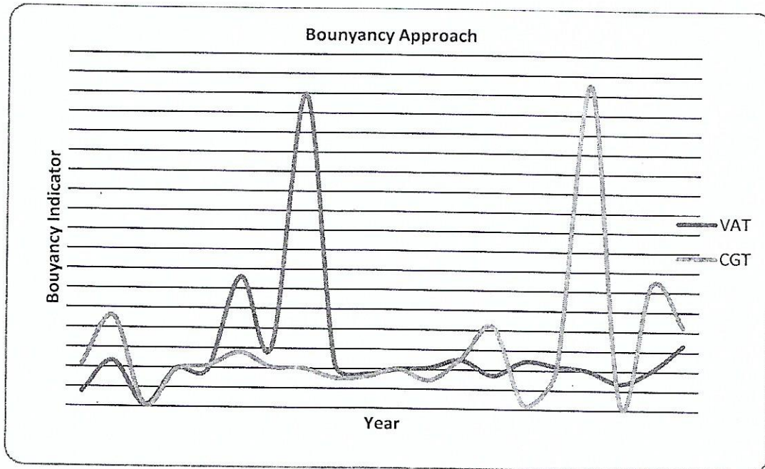
Figure 2: Diagrammatical Representation of VAT and CGT using Buoyancy Approach
