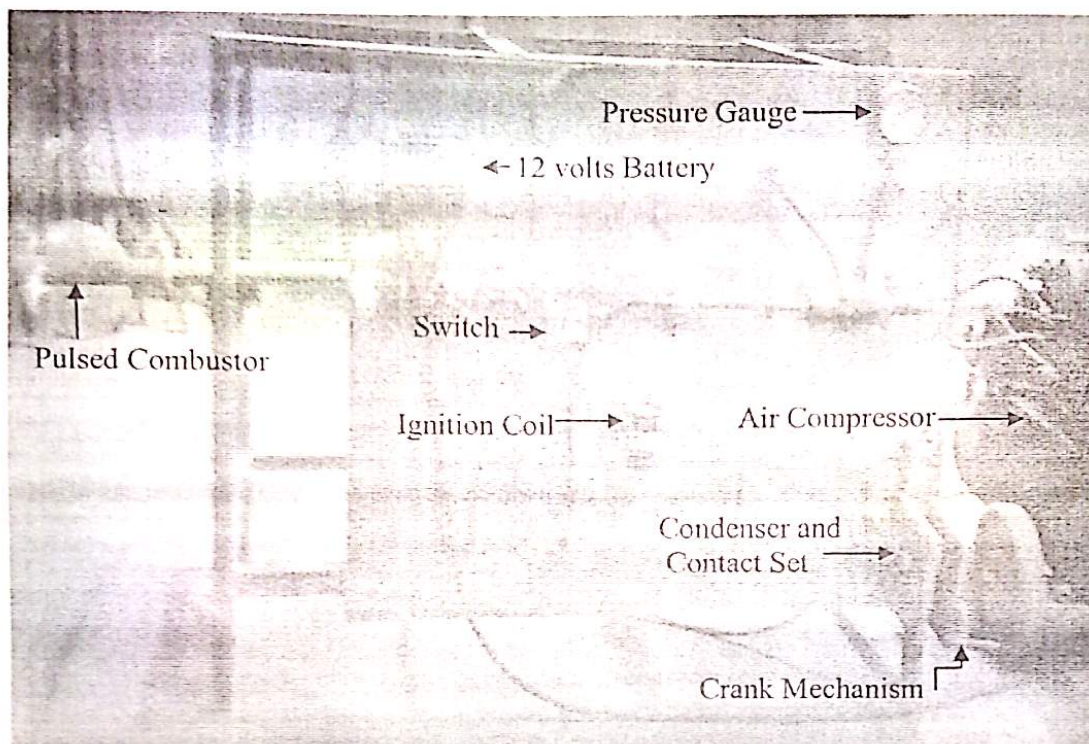
Figure 3: Photograph of the Experimental Rig Showing the Ignition System
