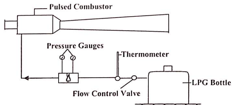
Figure 1: Schematic Diagram of the SNECMA-Lockwood Type Locally Fabricated Pulsed Combustor
