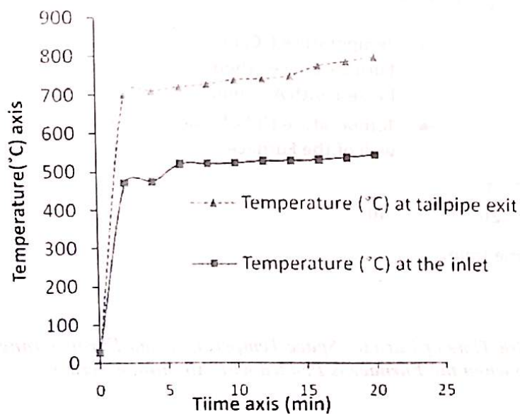
Figure 5: Variation with Time of Gas Temperature at Tailpipe Exit and Inlet Pipe of the Pulsed Combustor.
