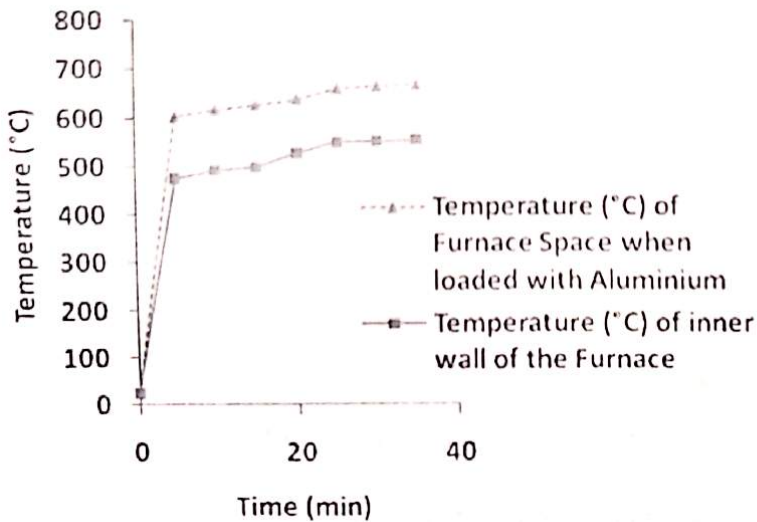
Figure 7: Variation with Time of Furnace Space Temperature and Furnace Inner Wall Temperature when the Furnace is Loaded with Aluminum Scraps.
