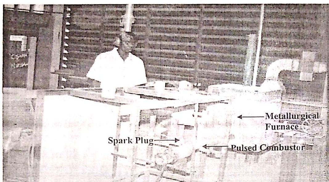
Figure 4: Photograph of the Experimental Rig Showing the Pulsed Combustor and Furnace in Operation
