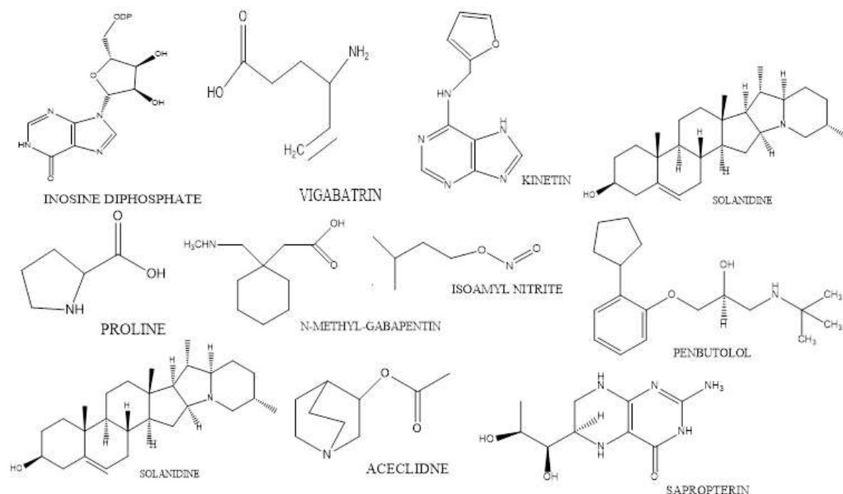
Fig 1: Structures of Volatile and Nonvolatile Compounds Identified in the Ethyl Acetate Extract of Trichoderma Harzianum with Antioxidant Properties
