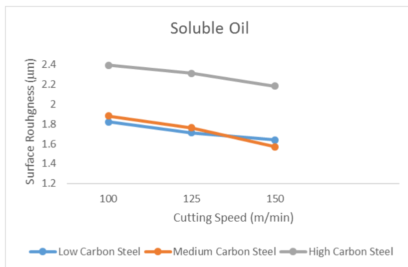
Figure 4: Surface Roughness at various Cutting Speeds (Cutting Fluid: soluble oil)
