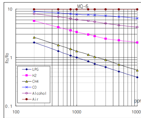
Figure 3. Sensitivity characteristics graph for MQ-6 gas sensor [30, 31]
