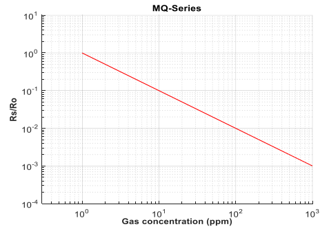
Figure 2. Hypothetical MQ-series sensor sensitivity characteristic curve
