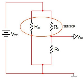
Figure 1. MQ-series gas sensor electrical equivalent circuit [30, 31]
