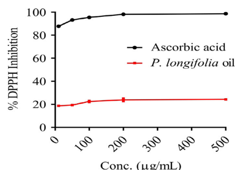
Fig. 2 DPPH anti-oxidant activities of ascorbic acid (control) and P. longifolia seed oil
