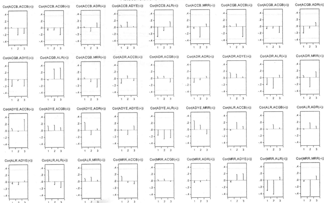
Figure 1: Autocorrelation Graphical Representation
