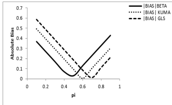
FIGURE 10. Absolute Bias for Mangat and Singh [23]; RRT at n=250 , x=106 , P=0.6 , T=0.1
