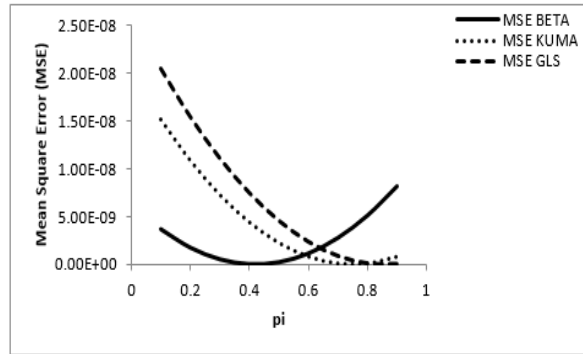
FIGURE 3. Mean Square Errors (MSEs) for Mangat and Singh [23]; RRT at n=25 , x=11 , P=0.6 , T=0.2
