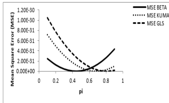
FIGURE 5. Mean Square Errors (MSEs) for Mangat and Singh [23]; RRT at n=100 , x=43 , P=0.6 , T=0.1
