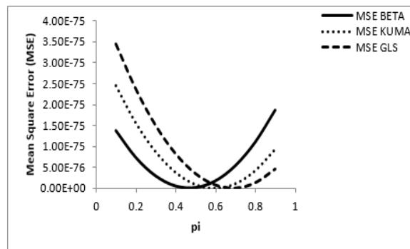
FIGURE 9. Mean Square Errors (MSEs) for Mangat and Singh [23]; RRT at n=250 , x=106 , P=0.6 , T=0.1
