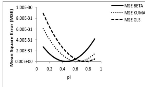
FIGURE 7. Mean Square Errors (MSEs) for Mangat and Singh [23]; RRT at n=100 , x=43 , P=0.6 , T=0.2
