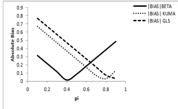
FIGURE 2. Graph showing the Absolute Bias for Mangat and Singh [23]; RRT at n=25 , x=11 , P=0.6 , T=0.1
