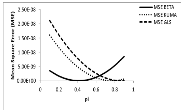
FIGURE 1. Graph showing the Mean Square Errors (MSEs) for Mangat and Singh [23]; RRT at n=25 , x=11 , P=0.6 , T=0.1
