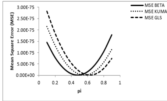
FIGURE 11. Mean Square Errors (MSEs) for Mangat and Singh [23]; RRT at n=250 , x=106 , P=0.6 , T=0.2
