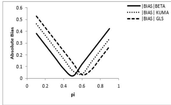
FIGURE 12. Absolute Bias for Mangat and Singh [23]; RRT at n=250 , x=106 , P=0.6 , T=0.2
