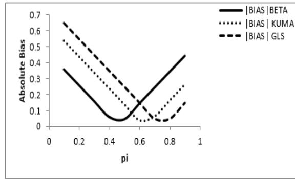
FIGURE 6. Absolute Bias for Mangat and Singh [23]; RRT at n=100 , x=43 , P=0.6 , T=0.1
