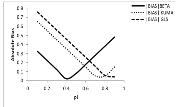
FIGURE 4. Absolute Bias for Mangat and Singh [23]; RRT at n=25 , x=11 , P=0.6 , T=0.2
