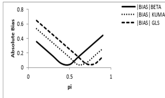
FIGURE 8. Absolute Bias for Mangat and Singh [23]; RRT at n=100 , x=43 , P=0.6 , T=0.2
