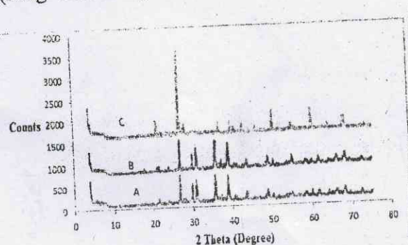
Figure 2: XRD pattern of as-synthesized catalyst (A) A-row (B) B-calcined (C) Cu modified
