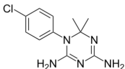
Figure 1: Structure of Cycloguanil
