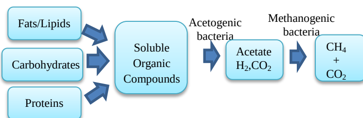
Figure 1: Schematic biochemical process stages of anaerobic digestion (Source: Achinas and Euverink, 2016)
