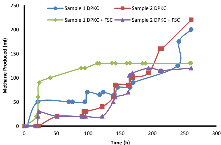
Figure 8: Cumulative methane production with time.
