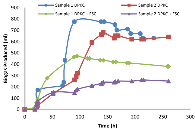
Figure 7: Cumulative biogas production with time.
