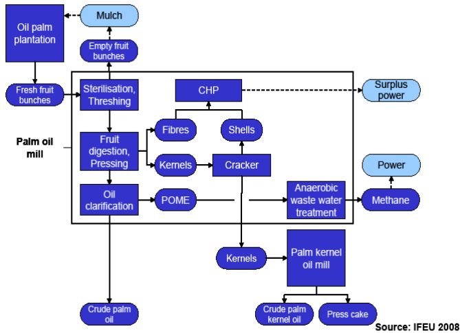
Figure 2: Processing of palm oil mill by-products and waste
