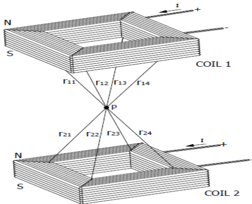
Fig. 2: Two Coils Arrangement
