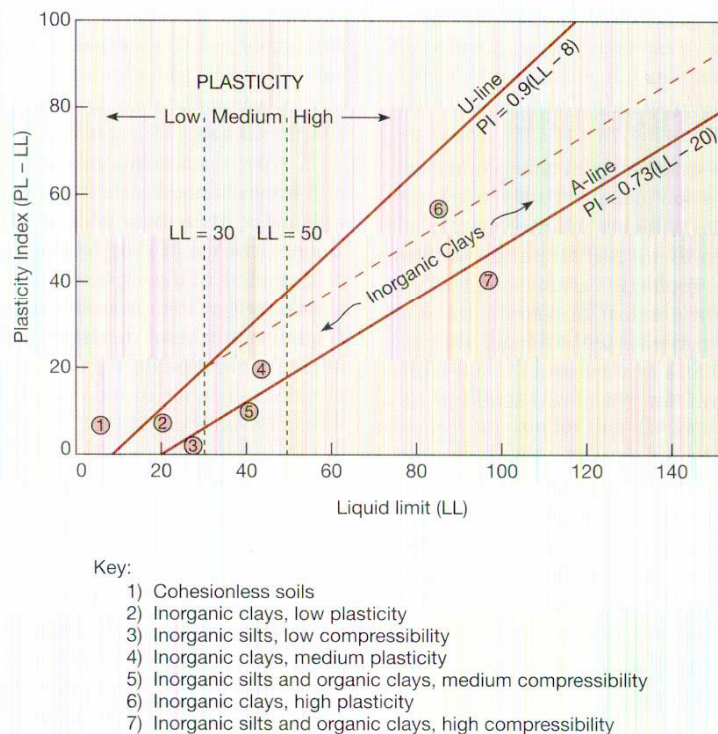
Fig. 1: Casagrande's Plasticity Chart
