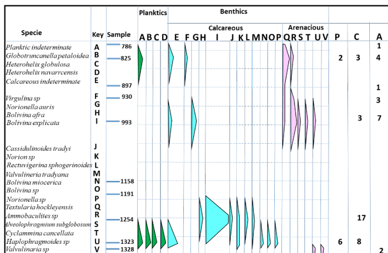
Fig. 4. Recovered planktonics and benthonics foraminifera and count/depth of species in the Agbabu-1 Well
