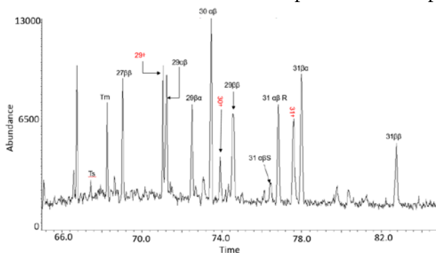
Fig. 13. m/z 191 mass chromatogram of sample Ar-145 showing the terpenoids distribution. Numbers refer to carbon numbers. ββ, βα, αβ, refer to the stereochemistry at the 14 and 21 carbon number respectively in the hopanes structure. Labels in red (e.g. 29†) are Hopenes.
