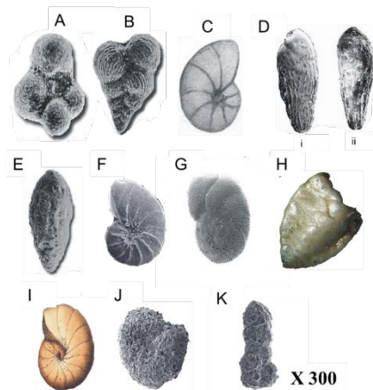
Fig. 3. Photomicrograph of some of the foraminifera identified. (A) Globotruncanella petaloidea (B) Heterohelix globulosa (C) Nonionella auris (D) Afrobolivina afra (E) Bolivina explicata (F) Nonion sp (G) Valvulineria sp (H) Textularia hockleyensis (I) Cyclammina cancellata (J) Haplophragmoides sp (K) Ammobaculites sp
