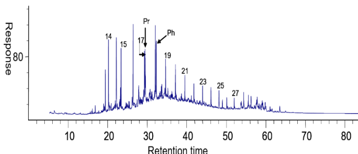
Fig. 10. A unimodal n -alkane envelope of sample Ar-145 maximizing at nC_{16} typical of a dominantly marine algae contribution to the organic matter. Note 14,15, etc. represents the n -alkane carbon numbers
