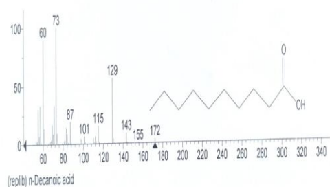
Decanoic acid
