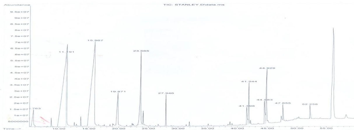
Figure 1. Mass spectrum of phytocomponents identified by GC-MS in the petroleum ether extracts of IGS.
