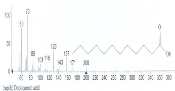
dodecanoic acid
