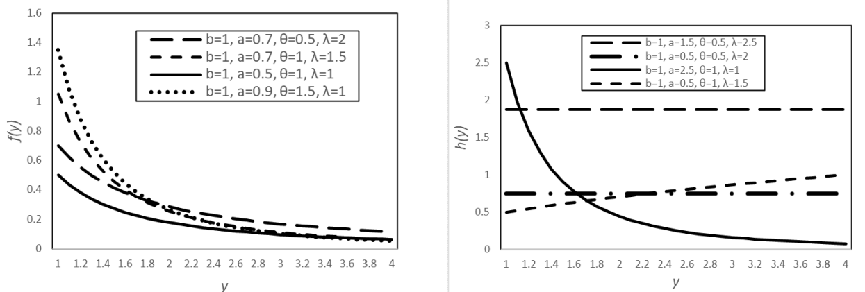
Figure 4: Plots of possible shapes of PDFs and HFs of EPT1-4.
