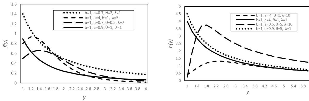
Figure 3: Plots of possible shapes of PDFs and HFs of EPT1-3.
