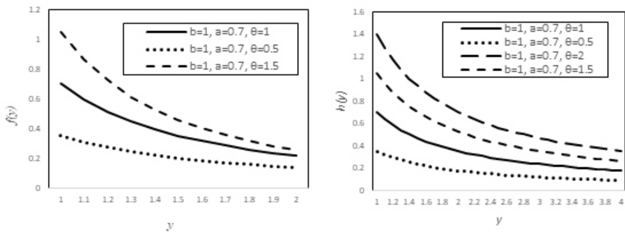
Figure 1: Plots of possible shapes of PDFs and HF of EPT1-1.
