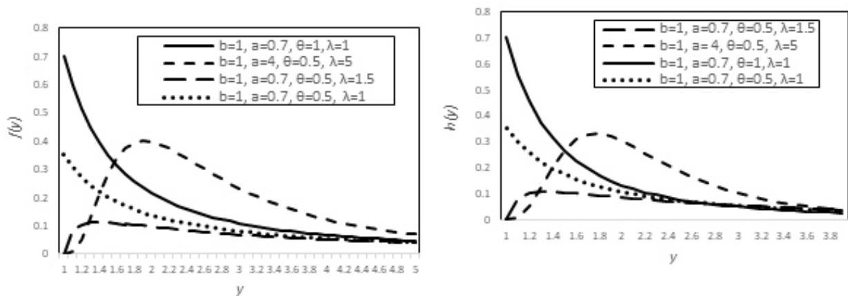
Figure 2: Plots of possible shapes of PDFs and HF of EPT1-2.
