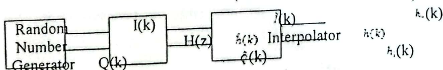
Figure 5: The Fading Sequence Generator
