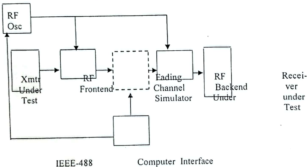
Figure 2: Simulator General Block Diagram
