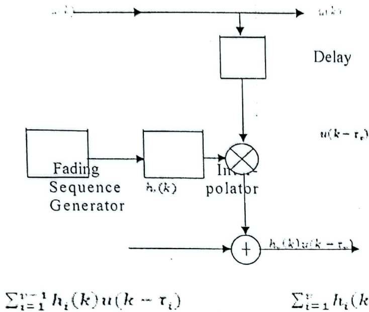
Figure 3: Simplified Simulator Board
