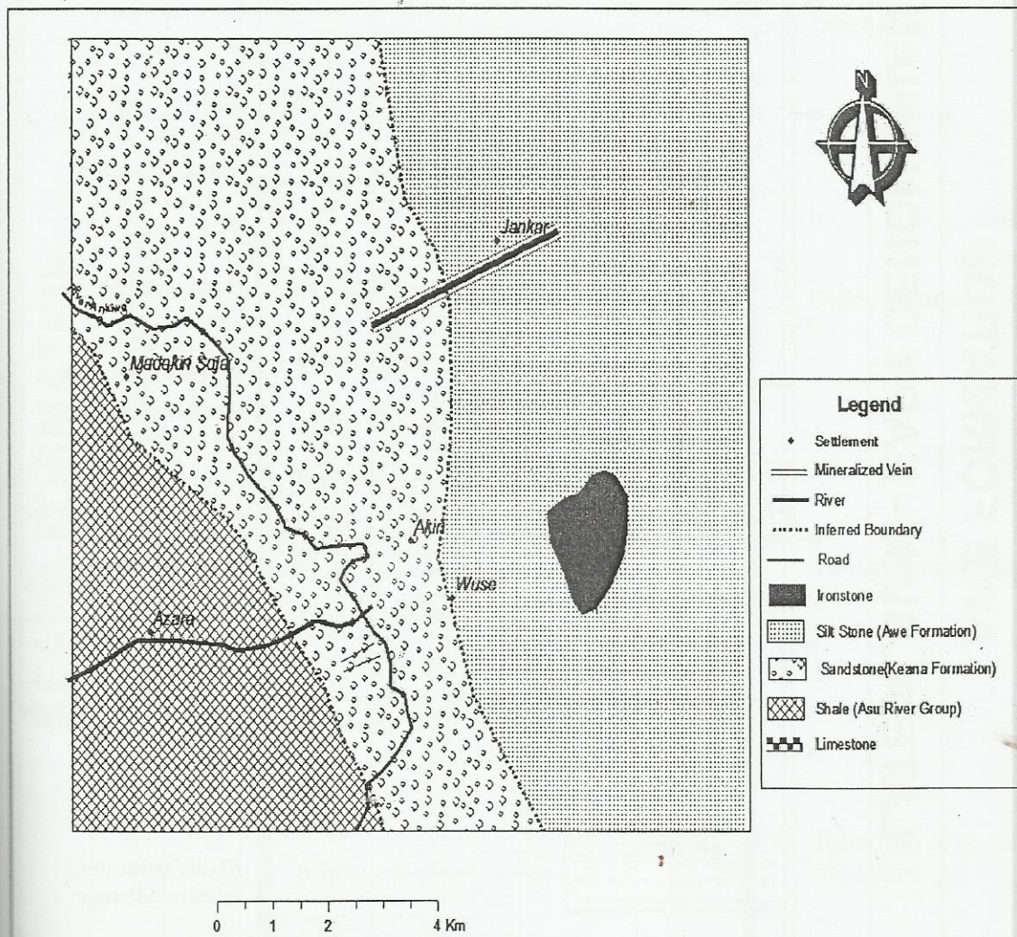
Fig. 2: Location Map of the Studied Area around Akiri, Wuse and Azara, Middle Benue Trough, Nigeria
