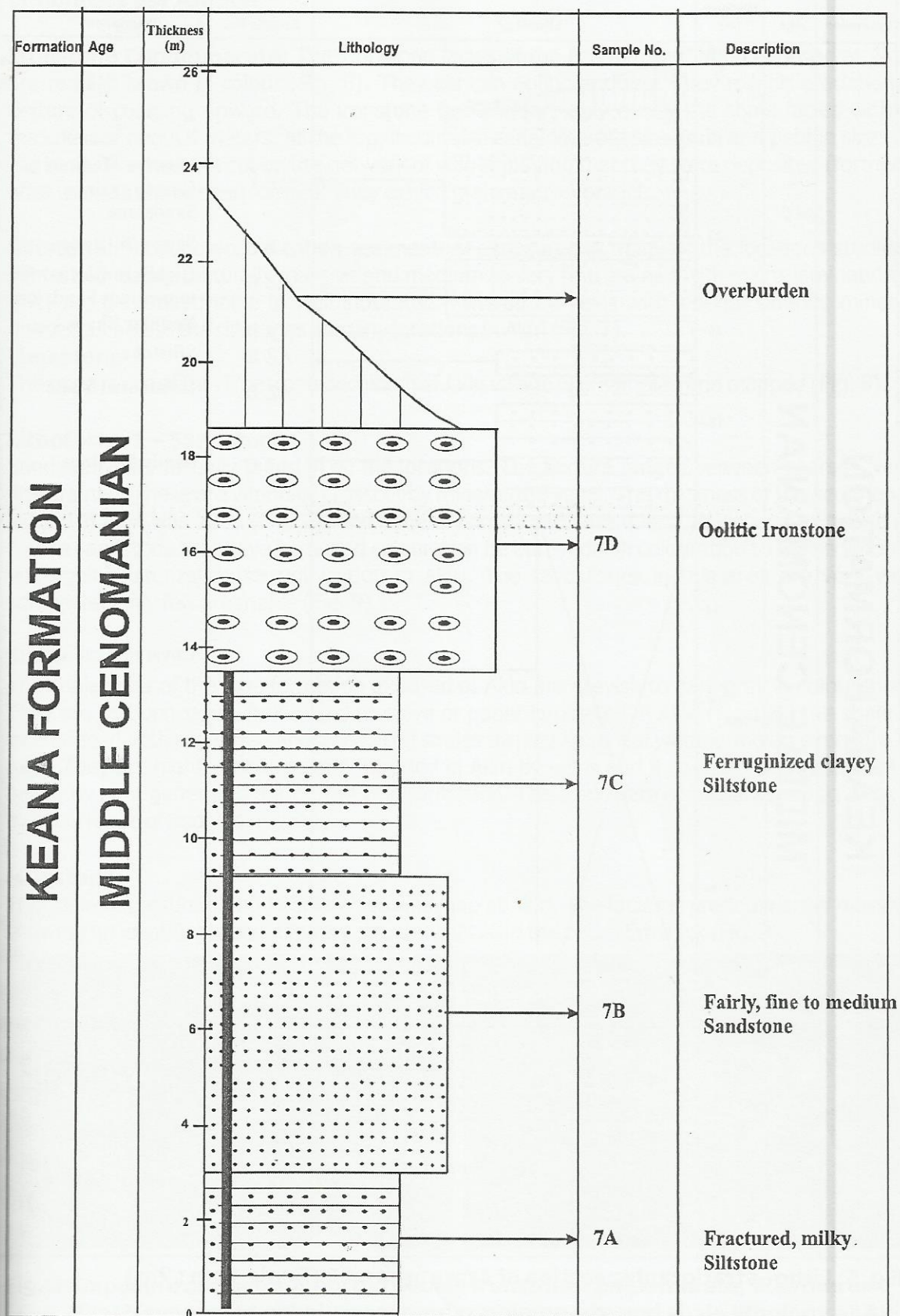
Fig. 4: Local Litho- stratigraphic section of Akiri pit 2 (Scale 1cm : 2m)
