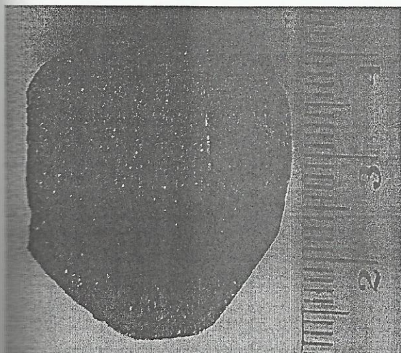
Fig. 22: (a) Laminated Mineralization in shale
