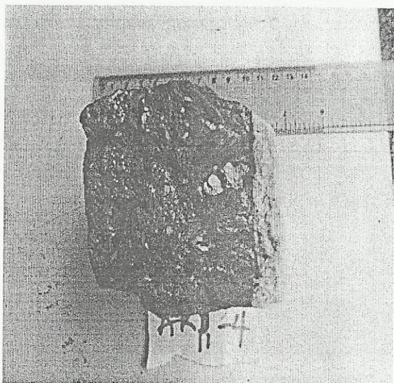
Fig. 18: Vein siderite within SE of Akiri showing disseminated chalcopryite core, siderite middle and outer quartz silification.
