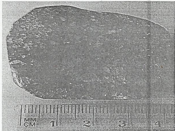
Fig. 21: Disseminated Sulphide ore in compacted sandstone and brecciated siderite
