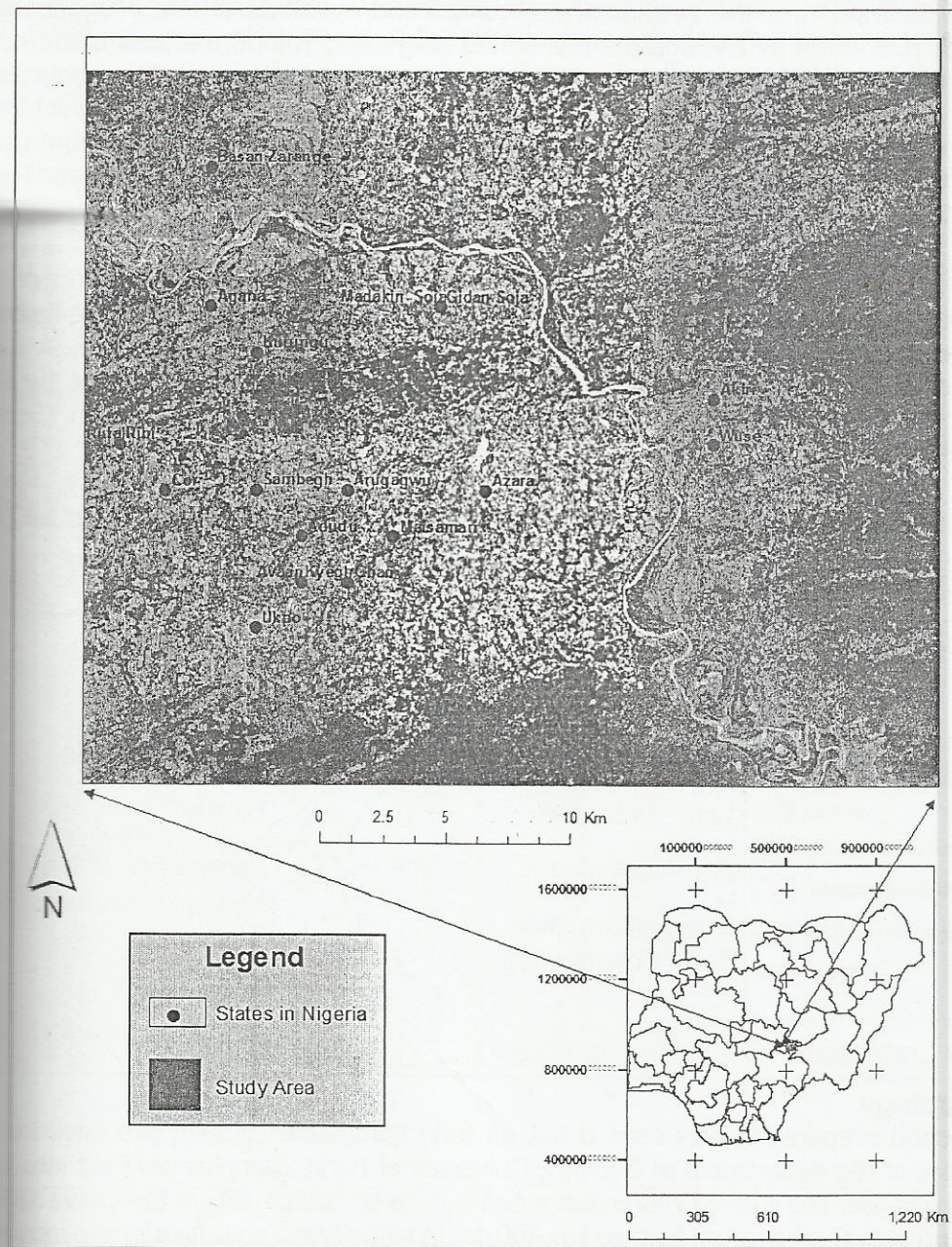
Fig. 1: Location map of Akiri, Nasarawa, Nigeria
