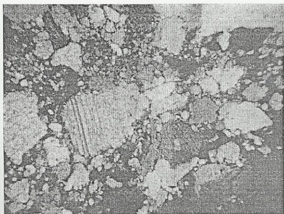
Fig.14: Thin section photomicrograph of well cemented medium-to coarse-grained sandstone
