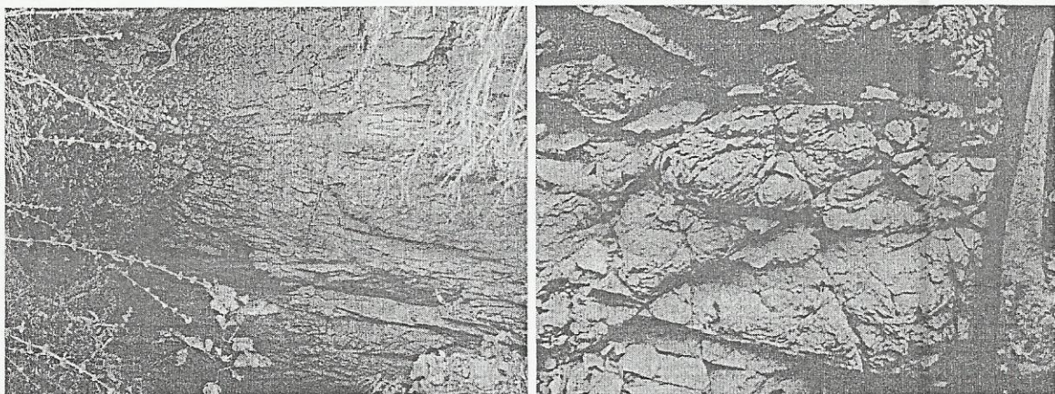
Fig. 10: Nodular shale within Eze Aku formation NE of Akiri.
