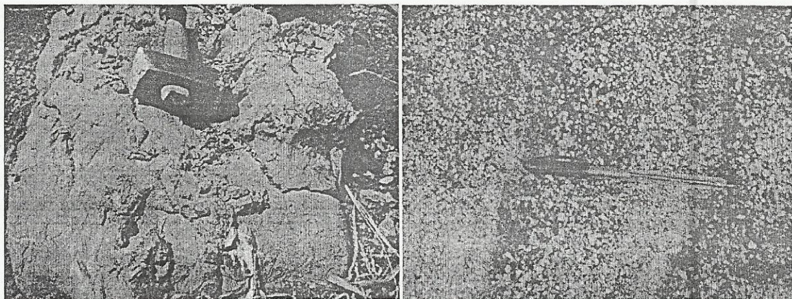
Fig.8: Highly indurated Limestone of Eze Aku Formation exposed at Jankar, 6 Km north of Akiri
