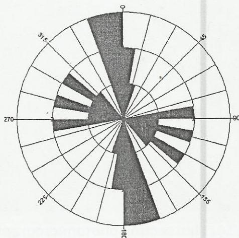
Fig. 12: Vein mineralization occupying steeply dipping fractures
