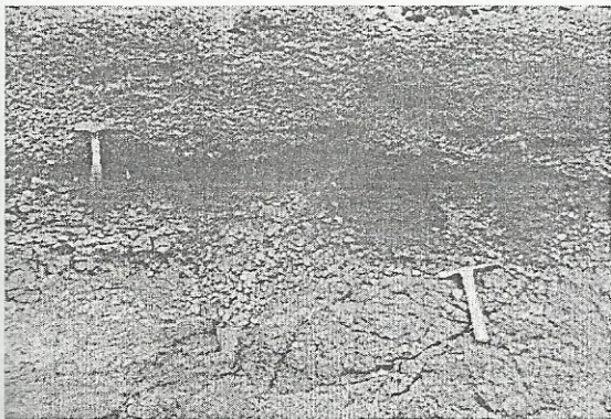
Fig. 6: Exposure of clast-supported pebbly ironstone conglomerate, Weathered Clast-supported pebbly ironstone conglomerate and shale lithology at Akiri pit 1.
