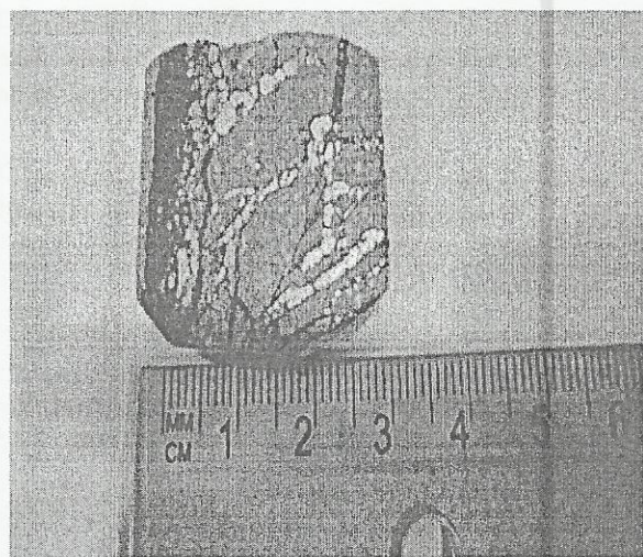
Fig. 21: Disseminated Sulphide ore in compacted sandstone and brecciated siderite
