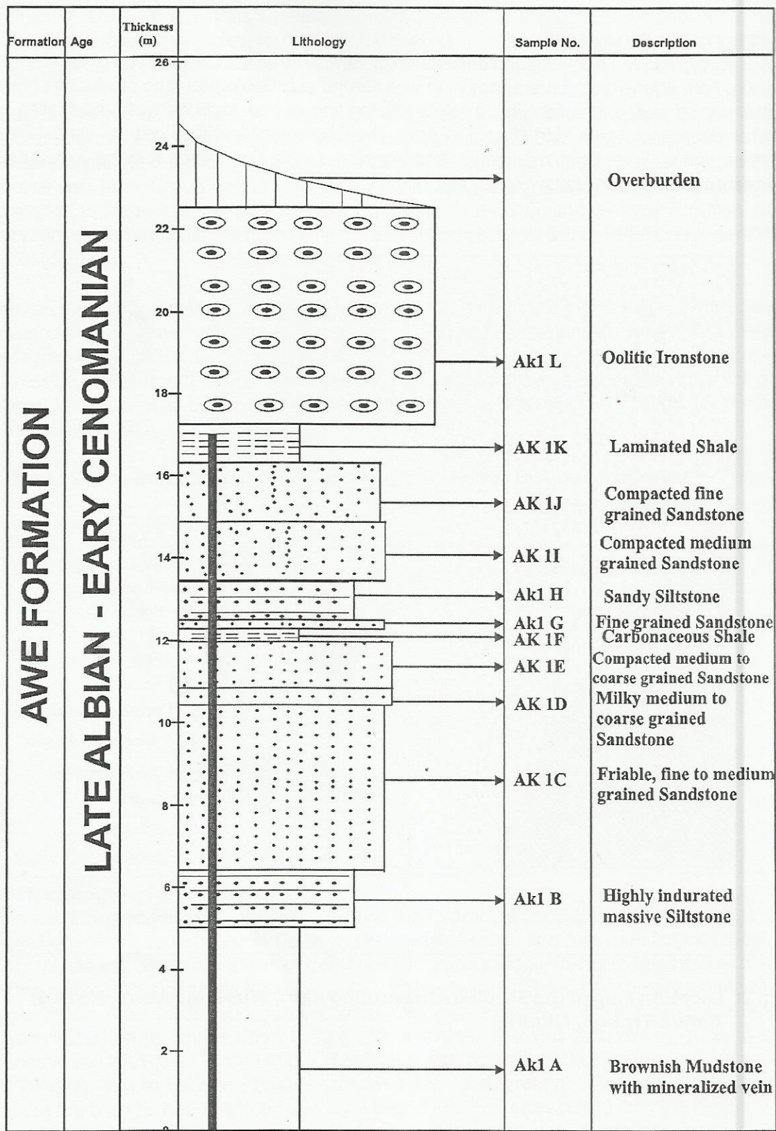
Fig. 3: Litho- Stratigraphic section of Akiri pit 1 (Scale 1.0cm : 2m)
