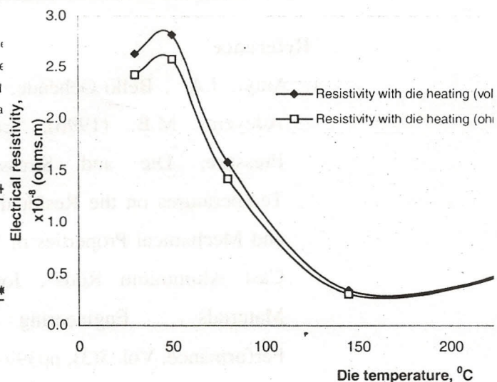
Figure 9 Comparison of calculated and direct resistance & resistivity of aluminium metal with pressure application
