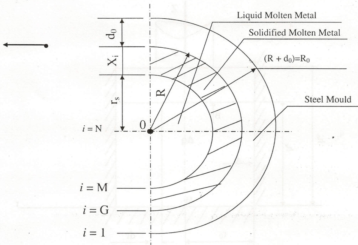
Figure 3: Schematic representation of solidification front in a cylindrical mould in one dimension (sectional view)
