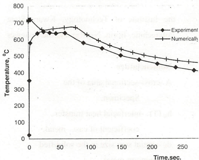
Figure 6 Typical comparison of the effect of applied pressure on temperature of aluminium metal ( P= (delay time=20 sec., retention time=55 s
