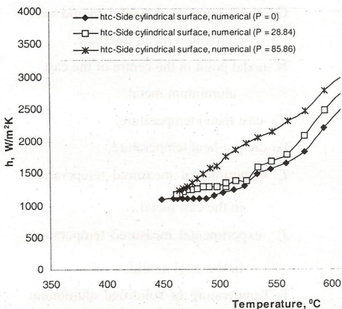
Figure 7 Typical effects of pressure application on solidifying temperature of the side cylindrical numerical method
