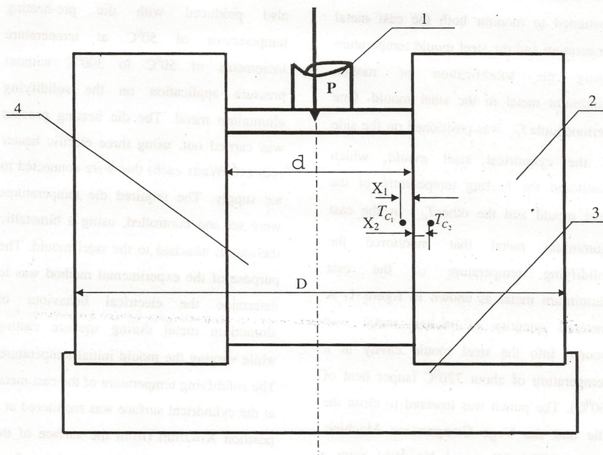
Figure 1 Schematic diagram of squeeze casting test rig
