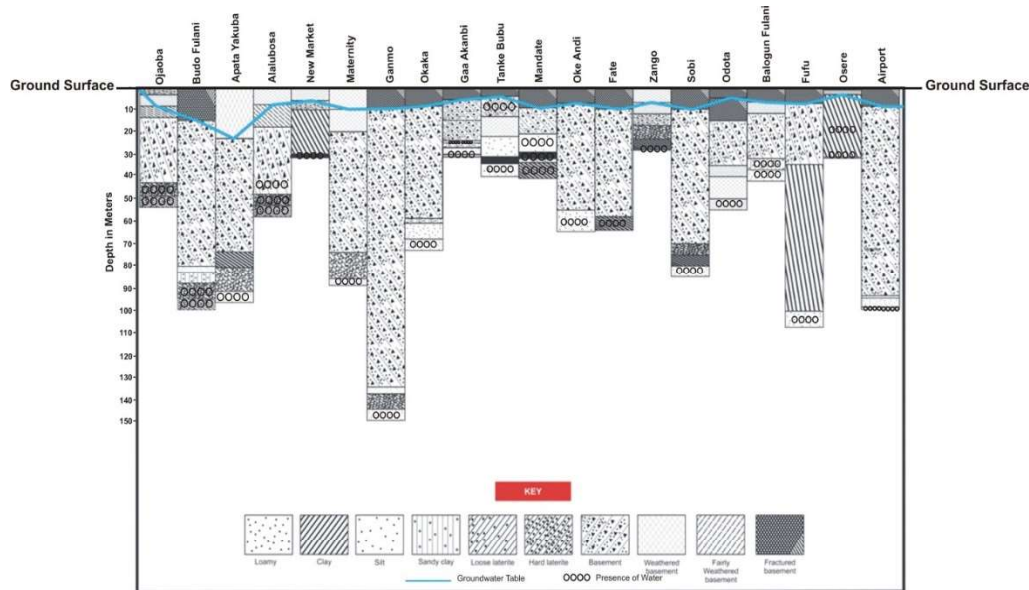
Fig. 3. Downhole Lithological Logs of Studied Boreholes.
