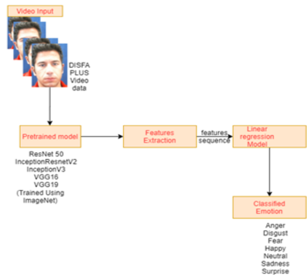
Fig 1. Transfer learning model diagrams
