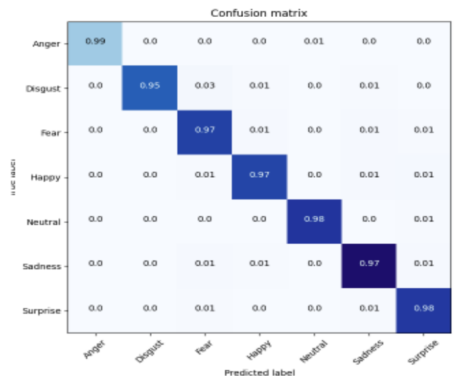
Fig 2: Confusion matrix for VGG19 test result
