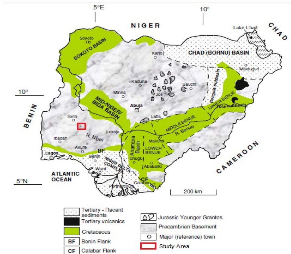
Fig. 2 Geology map of Nigeria showing the study area (Modified after Obaje et al. 2009)
