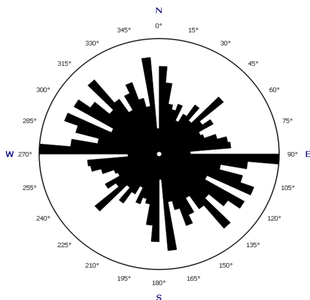
Fig. 7 General orientation of lineaments within the study area
