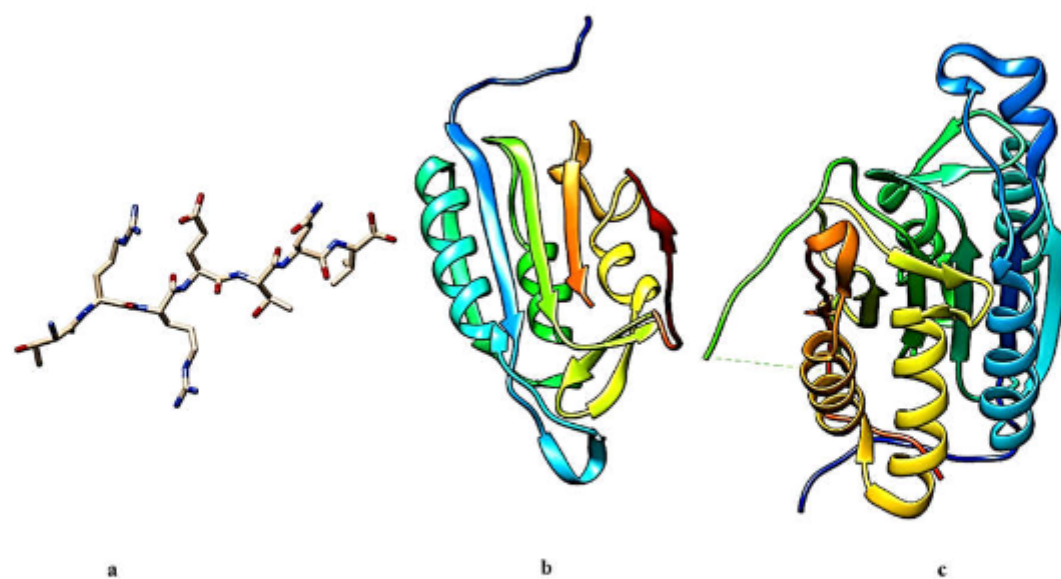
Fig. 1. 3D structures of (a) HPV 16 E6; (b) Caspase -3; (c) Caspase -8
