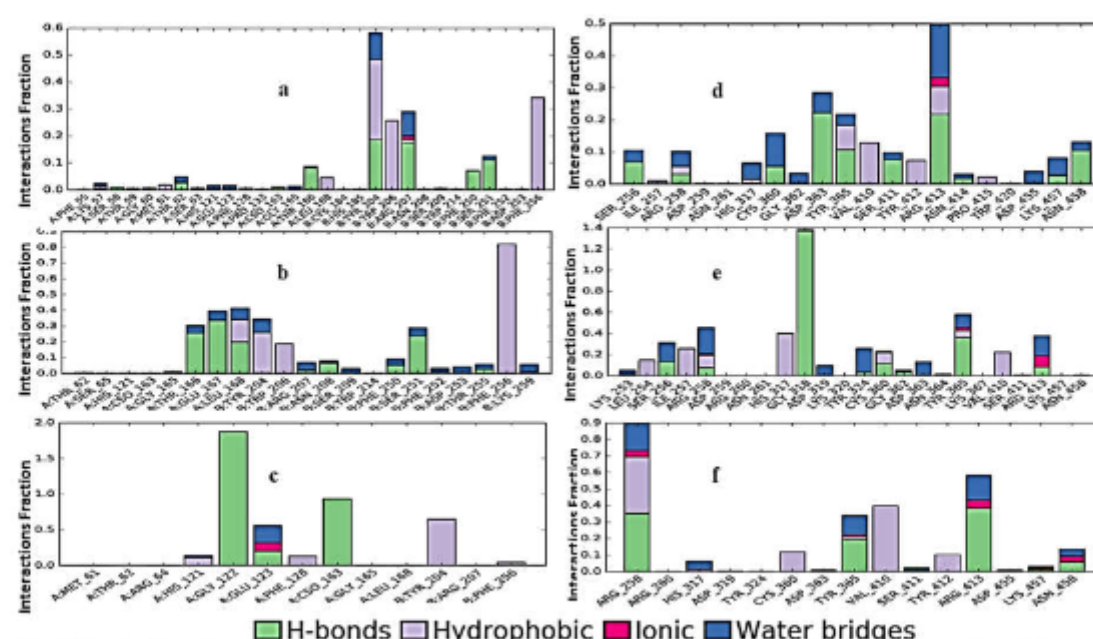
Fig. 9. Protein-ligand interactions with amino acids at the binding sites of caspases -3 and -8 in the presence of a and d – Carnosol; b and e – Luteolin; c and f: Melphalan
