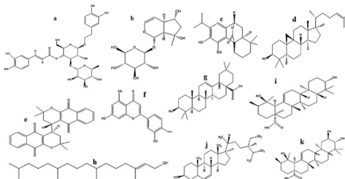
Fig. 2. 2D structures of (a) Acteoside (b) Ajugol (c) Carnosol (d) Cycloartenol (e) Dilapachone (f) Luteolin (g) Oleanolic acid (h) Phytol (i) Pomolic acid (j) Sitosterol (k) Tormentic acid
