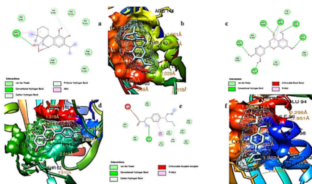
Fig. 3. 2D and 3D structures of a and b: Camosol-caspase-3; c and d: Luteolin-caspase-3; e and f: Melphalan-caspase-3
