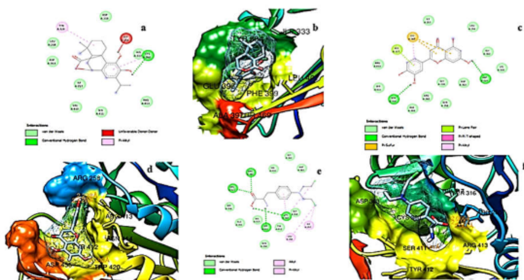
Fig. 4. 2D and 3D structures of a and b: Camosol-caspase-8; c and d: Luteolin-caspase-8; e and f: Melphalan-caspase-8
