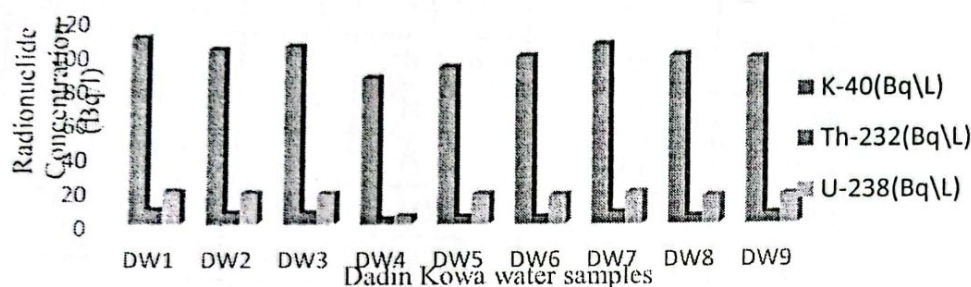
Figure 3: Activity Concentration of ^{40}\text{K} , ^{238}\text{U} and ^{232}\text{Th} in the water samples
