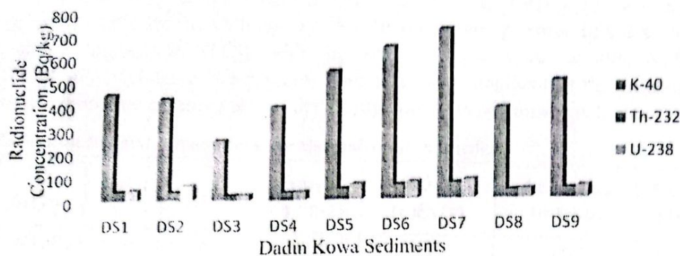
Figure 2: Activity Concentration of ^{40}\text{K} , ^{238}\text{U} and ^{232}\text{Th} in sediment samples
