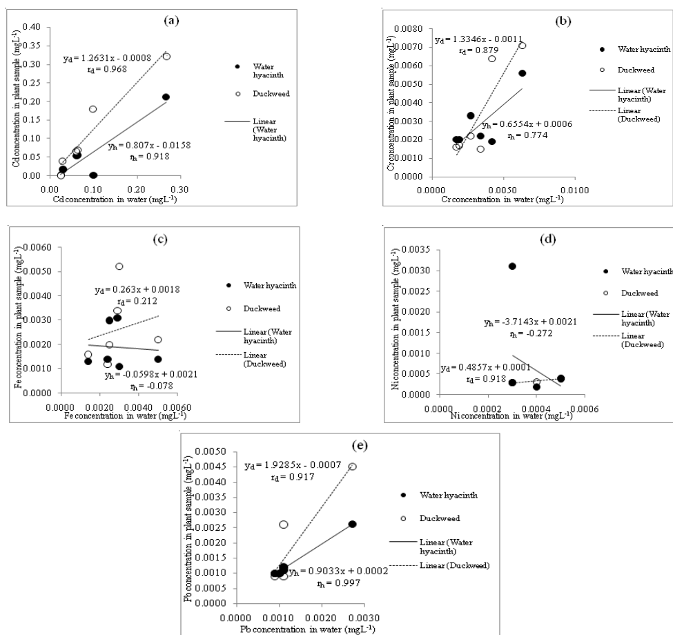
Fig. 2 Scattered graphs of (a) Cadmium (b) Chromium (c) Iron (d) Nickel and (e) Lead levels in duckweed and water hyacinth against their respective concentrations in water samples.
