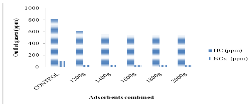
Fig 1: Gas effluent quality after passing through a combination of coconut shell activated carbon and charcoal
