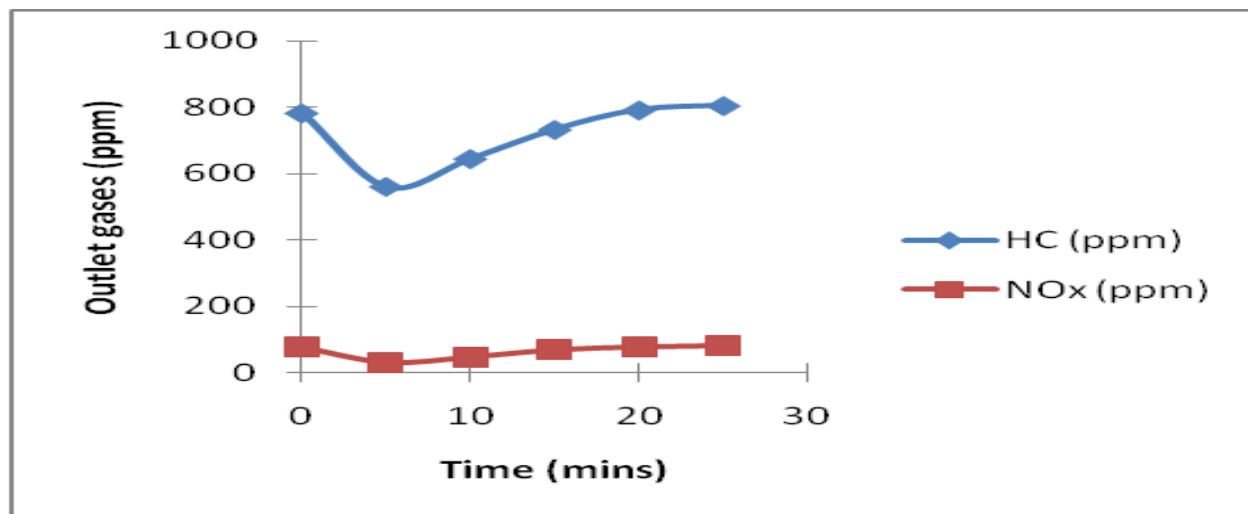
Fig 7: Breakthrough curves for HC and NO x
