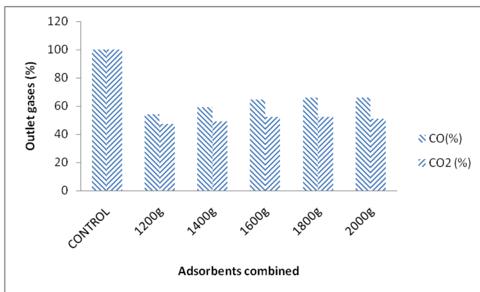
Fig 4: Percentages of the gas effluent removed after passing through a combination of coconut shell activated carbon and charcoal
