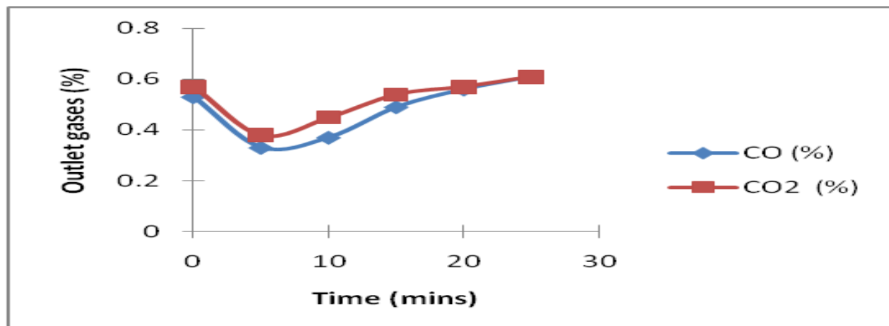
Fig 8: Breakthrough curves for CO and CO 2
