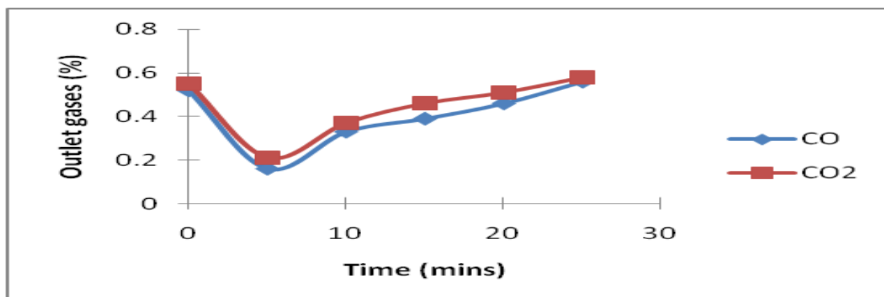
Fig 10: Breakthrough curves for CO and CO 2
