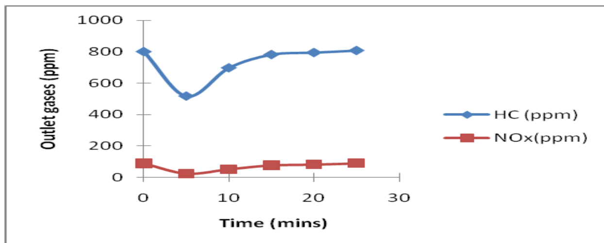
Fig 9: Breakthrough curves for HC and NO x
