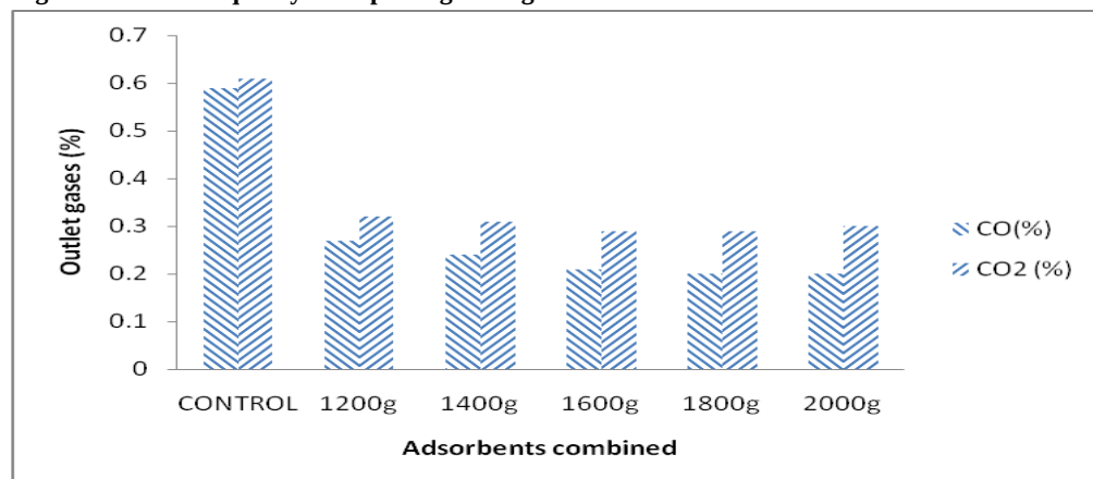
Fig 2: Gas effluent quality after passing through a combination of coconut shell activated carbon and charcoal
