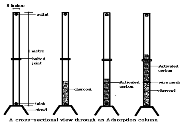
Fig 1: Schematic representation of the adsorption column
