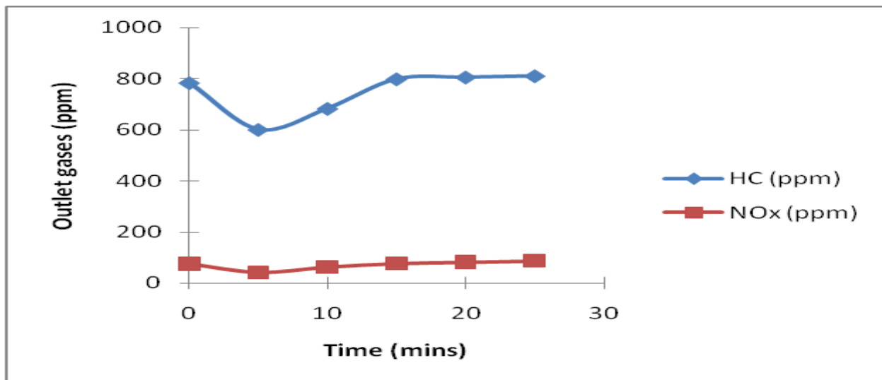
Fig 5: Breakthrough curves for HC and NO x
