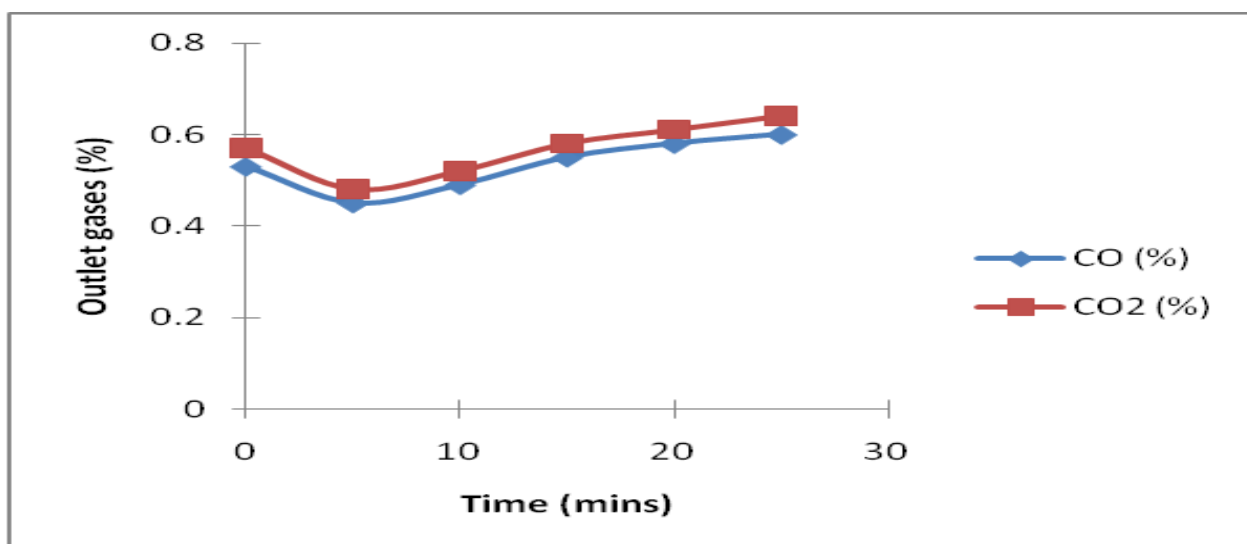
Fig 6: Breakthrough curves for CO and CO 2
