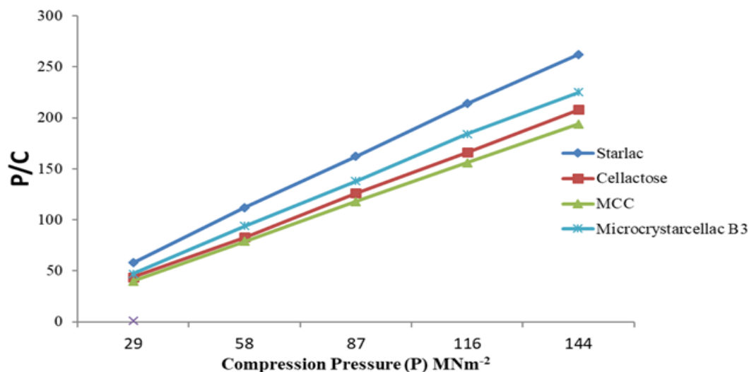
Fig. 5: Kawakita analysis of compacts P/C vs Compression pressure P (MNm -2 ) of MSCL B3, Starlac®, and Cellactose® placebo tablets
