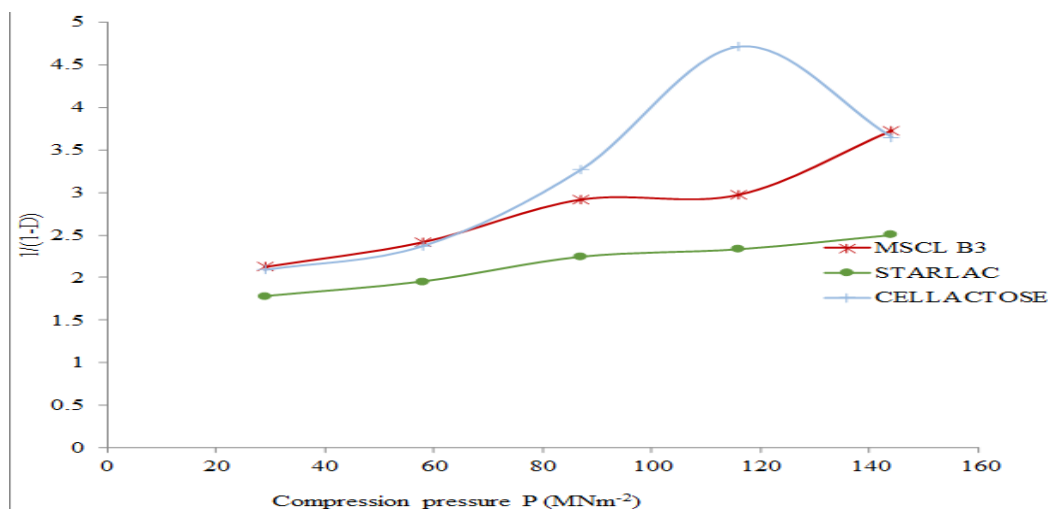
Fig. 4: Heckel's analysis of compact of microcrystalline cellulose (B3), Starlac, Cellactose,
