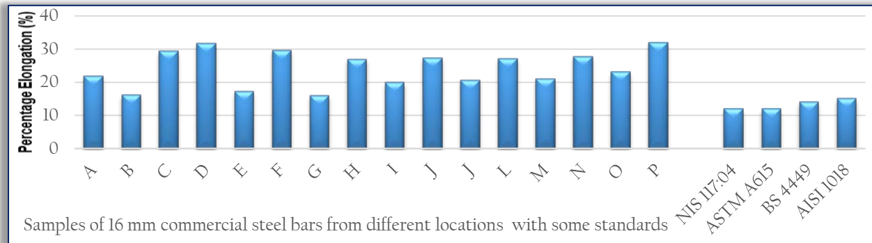
Figure 12: Percentage elongations of various 16 mm commercial reinforcement steel bars and standards
