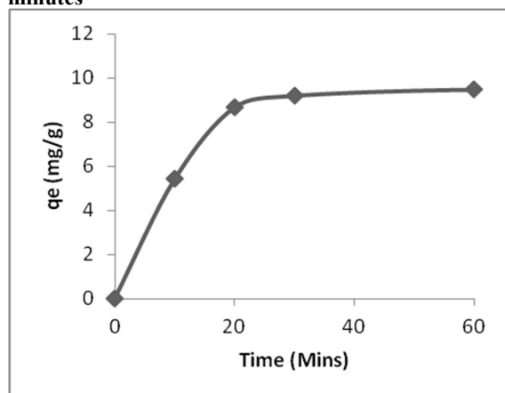
Figure 6: Effect of contact time on the adsorption of anthracene over [Cu(INA) 2 ] MOFs at 32 ± 2 °C, Concentration = 20 mg/L, pH = 4.99, speed = 168 rpm, time = 60 minutes
