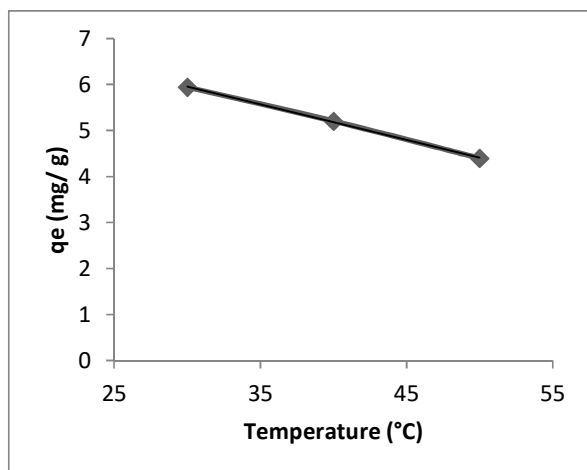
Figure 5: Effect of temperature on the adsorption of anthracene over [Cu(INA) 2 ] MOFs at Concentration = 20 mg/L, pH = 4.99, speed = 168 rpm, time = 30 minutes
