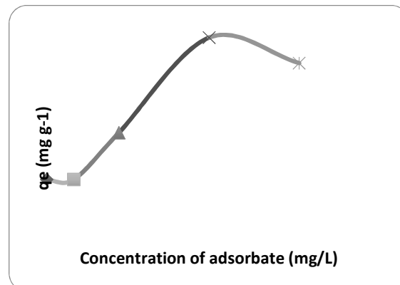
Figure 8: Effect of initial conc. on the adsorption of anthracene over [Cu(INA) 2 ] MOFs at 32 \pm 2 °C, pH of 4.99, 168 rpm, time = 30 minutes
