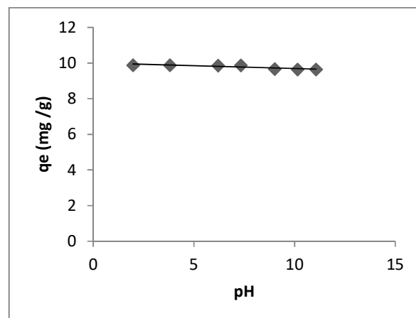
Figure 3: Effect of pH on the adsorption of anthracene over [\text{Cu}(\text{INA})_2] MOFs. Concentration = 20 mg/L, temperature = 32 \pm 2^\circ\text{C} , speed = 168 rpm, time = 30 minutes
