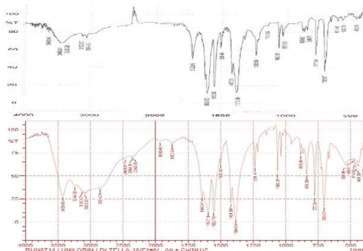
Figure 1: FTIR spectra of a) [Cu(INA) 2 ] MOFs b) [Cu(INA) 2 ] MOFs after adsorption of Anthracene
