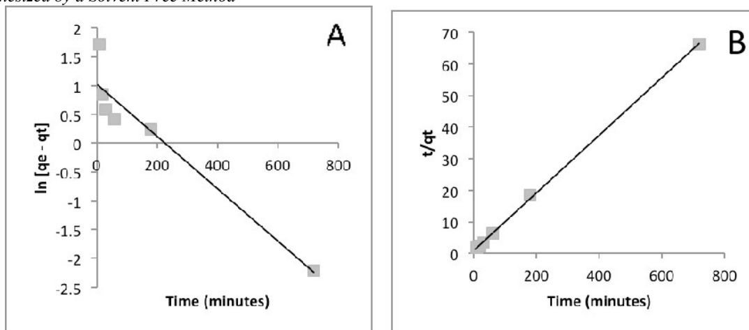
Figure 7: (A) Pseudo-first-order kinetic plot of anthracene (B) Pseudo-second-order kinetic plot of anthracene
