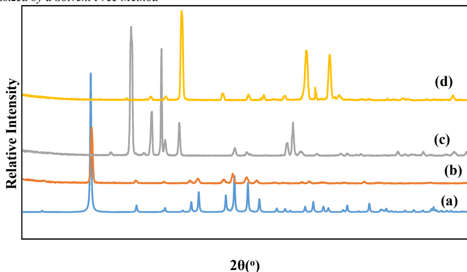
Figure 2: Comparison of XRD pattern of [\text{Cu}(\text{INA})_2] MOFs and reactants (a) Simulated patterns of [\text{Cu}(\text{INA})_2] from the single crystal data (b) Synthesized [\text{Cu}(\text{INA})_2] (c) Copper acetate (d) Isonicotinic acid
