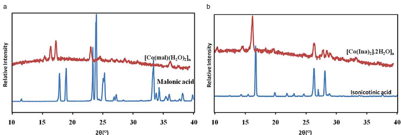
Fig. 3 – (a) PXRD pattern of malonic acid and [\text{Co}(\text{mal})]\cdot 2\text{H}_2\text{O} (1). (b) PXRD pattern of isonicotinic acid [\text{Co}(\text{Ina})_2]\cdot 2\text{H}_2\text{O} (2).
