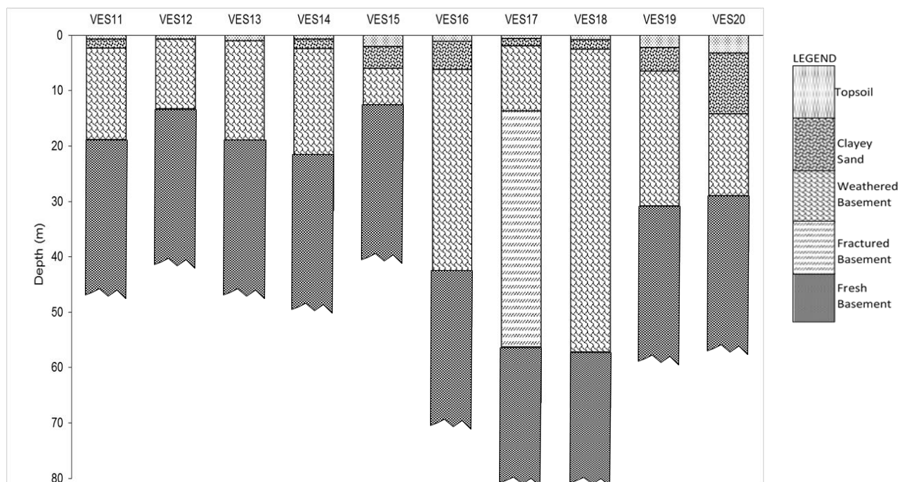
Figure 5: Geoelectric cross-sections of study area
