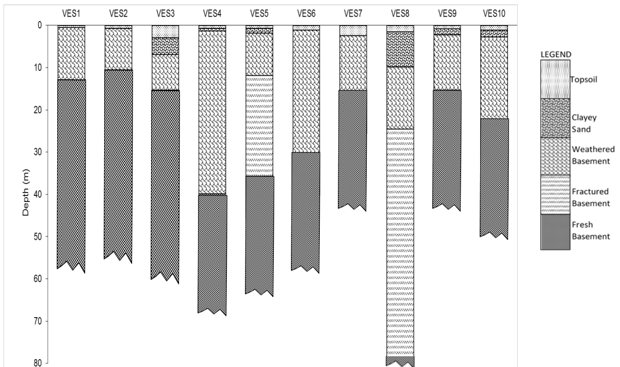
Figure 4: Geoelectric cross-sections of study area
