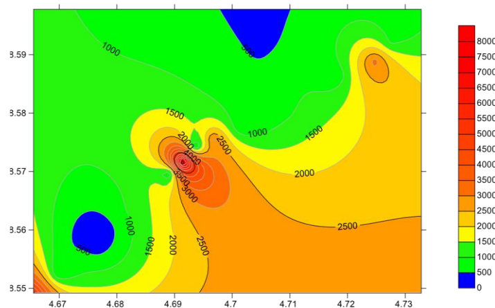
Figure 7e: Contour Resistivity Layer 5
