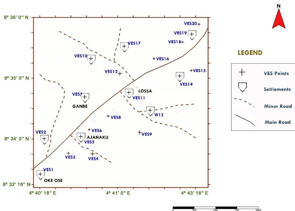
Figure 2: Location map of study area showing VES points
