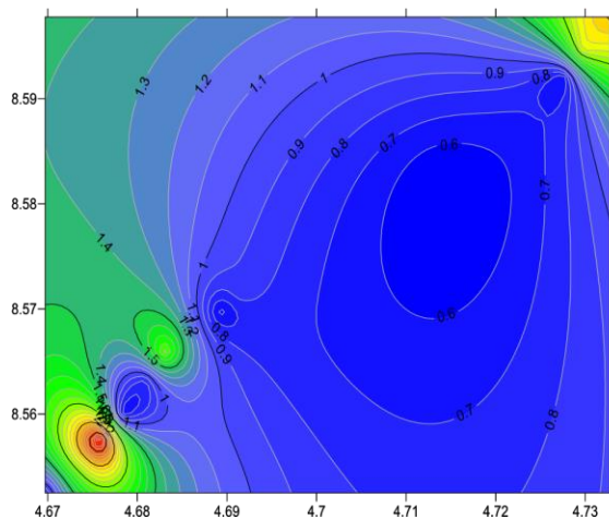
Figure 7a: Contour Resistivity Layer 1
