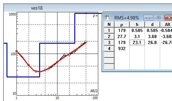
Figure 3d: Curve Type HA.
