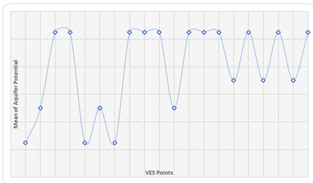
Figure 8: Aquifer potential pattern in study area
