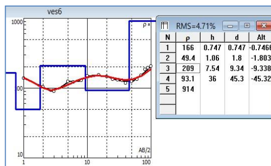
Figure 3b: Curve Type HKH.
