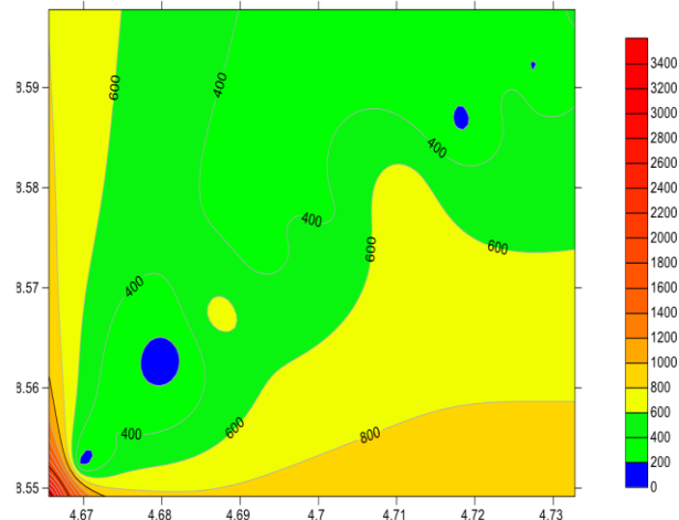
Figure 7d: Contour Resistivity Layer 4
