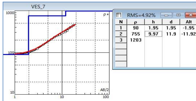
Figure 3e: Curve Type A
