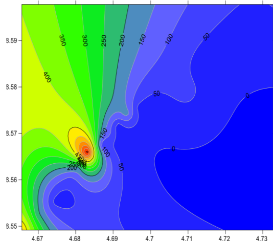
Figure 7c: Contour Resistivity Layer 3
