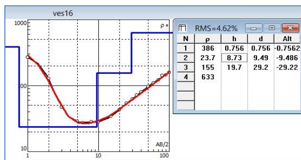
Figure 3a: Curve Type H.
