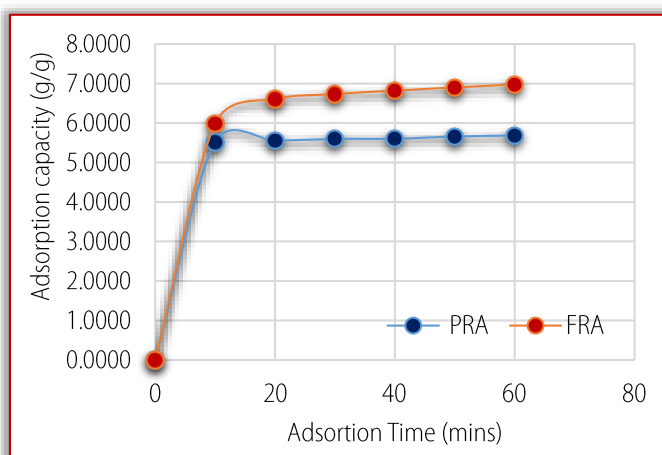
Figure 8: Effect of adsorption time of PRA and FRA on Diesel Oil
