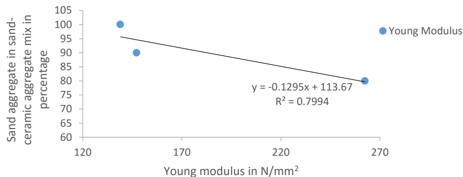
Figure 16: Aggregate mix ratio and Young's modulus nexus
