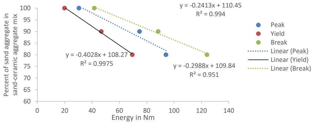
Figure 12: Aggregate mix ratio and energy applied nexus
