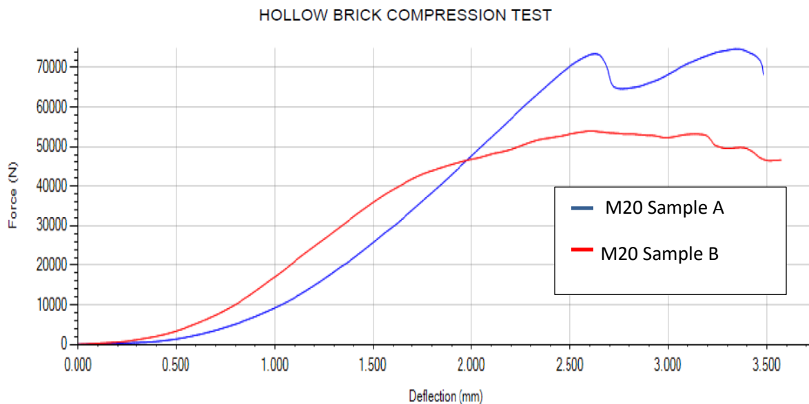
Figure 9: Stress strain curve for hollow block with 20% ceramic ware waste hollow block
