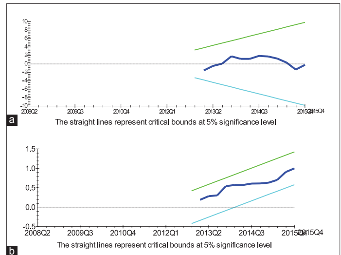
Figure 1: Malaysia. (a) Plot of cumulative sum of recursive residuals. (b) Plot of cumulative sum of squares of recursive residuals
