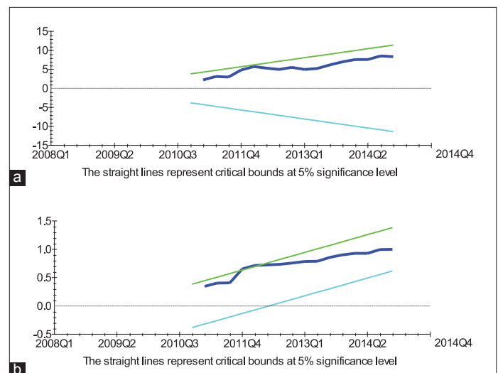
Figure 3: Bahrain. (a) Plot of cumulative sum of recursive residuals. (b) Plot of cumulative sum of squares of recursive residuals
