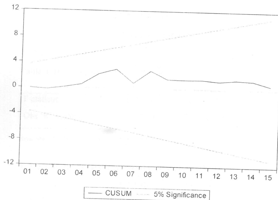
Fig. 1 Cumulative Sum of Recursive Residuals
