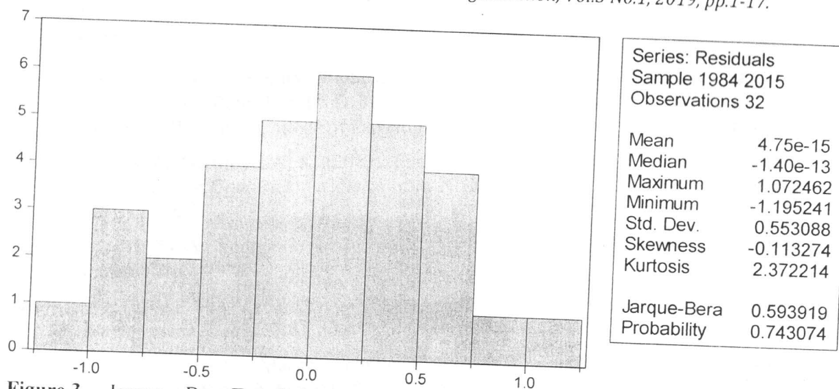
Figure 3 Jarque – Bera Test for Normality
