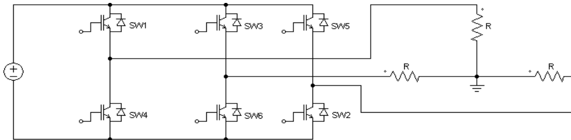
Fig. 2. The inverter switching logic circuit
