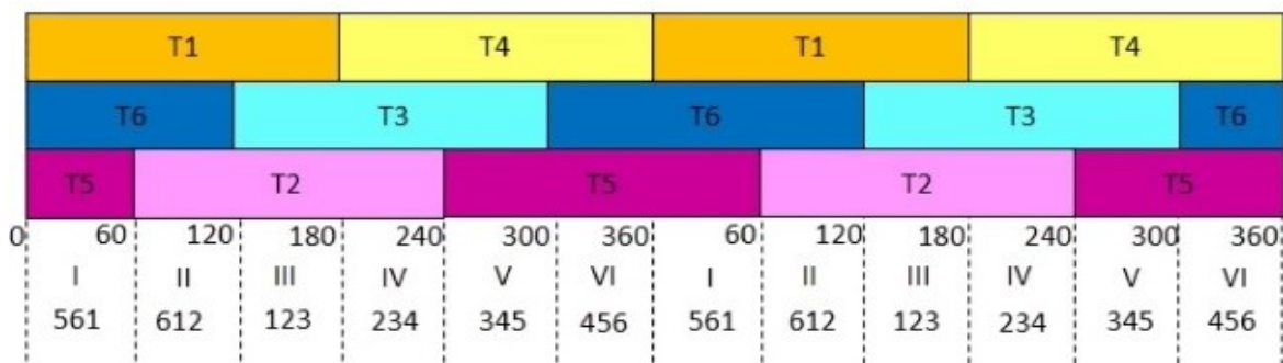
Fig. 3. The circuit pattern operation and the IGBT steps ON operations
