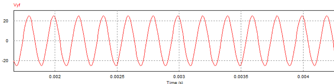
Fig. 14. Yellow phase output voltage of the inverter with innovative LC filter
