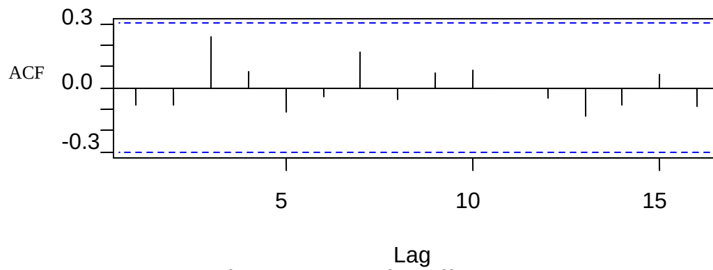
Figure 6: Plot of Autocorrelation for Differenced Electricity Consumption
