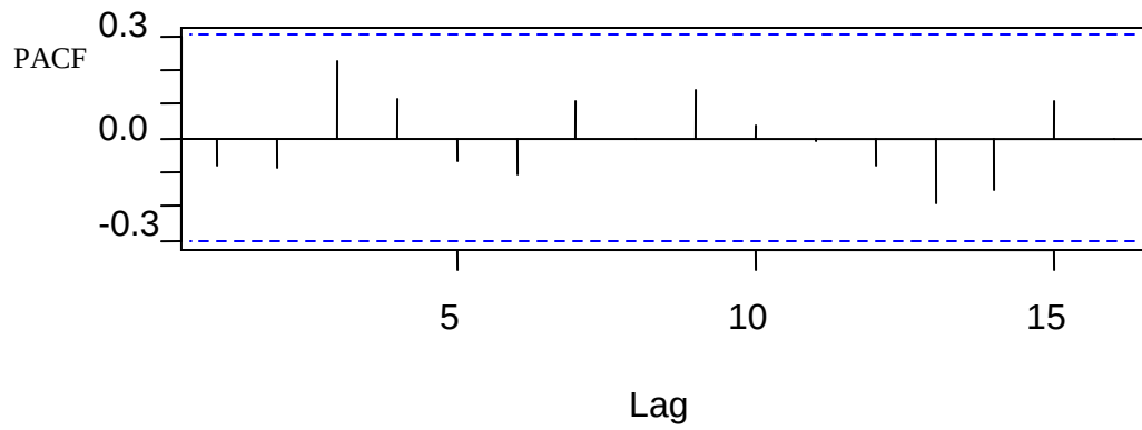
Figure 8: Plot of Partial Autocorrelation for Differenced Electricity Consumption
