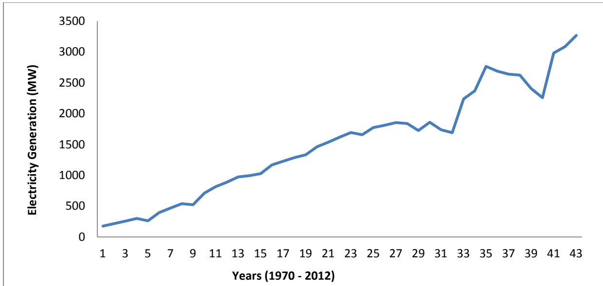
Figure 1: Time Plot for the Electricity Generation
