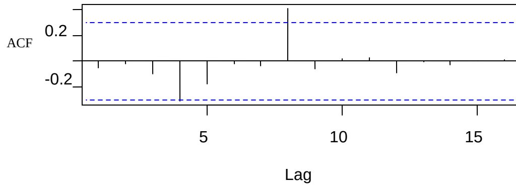
Figure 5: Plot of Autocorrelation for Differenced Electricity Generation
