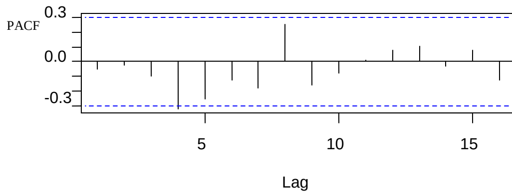
Figure 7: Plot of Partial Autocorrelation for Differenced Electricity Generation
