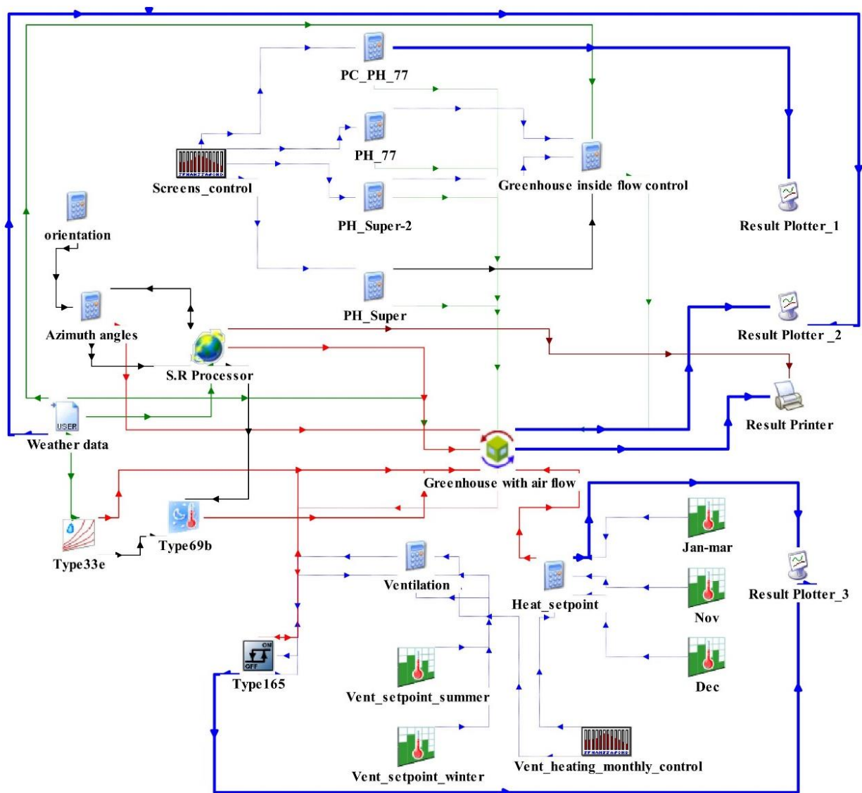
Figure 2: Typical BES model of a multi-span greenhouse in TRNSYS Simulation Studio (Rasheed et al., 2020b).
