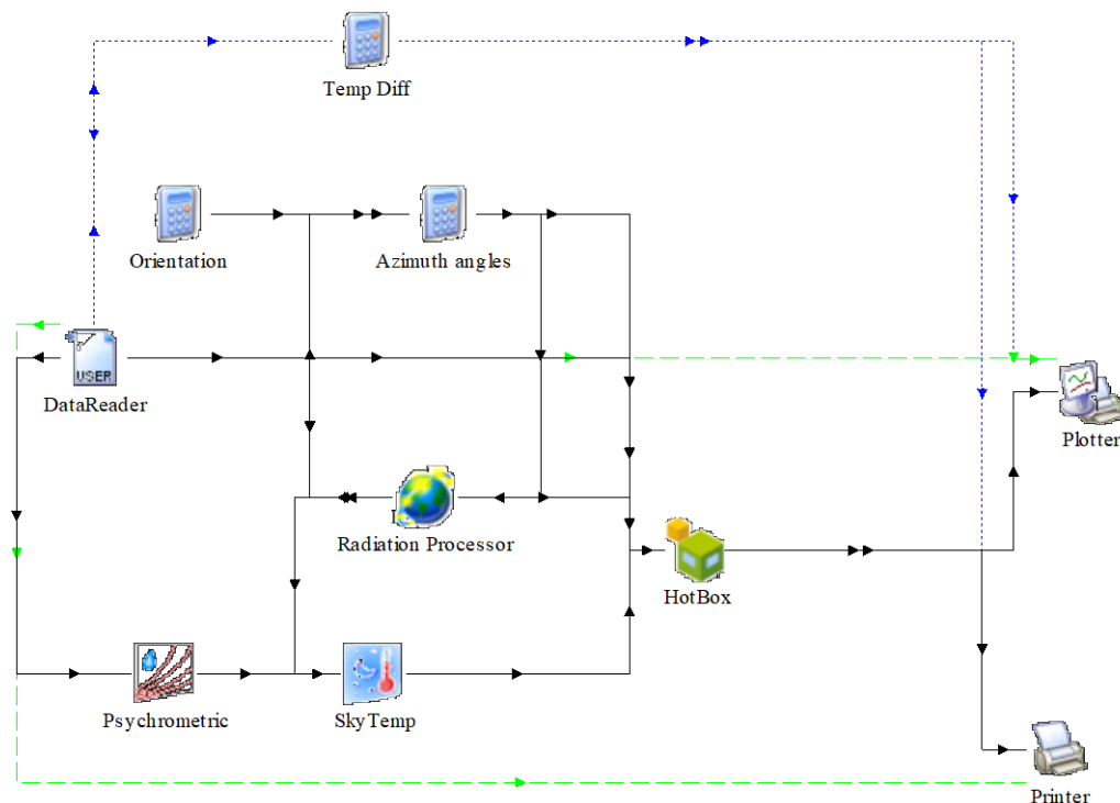
Figure 3. TRNSYS simulation for the determination of the U-value of greenhouse cover materials (Rabiu et al. , 2022).
