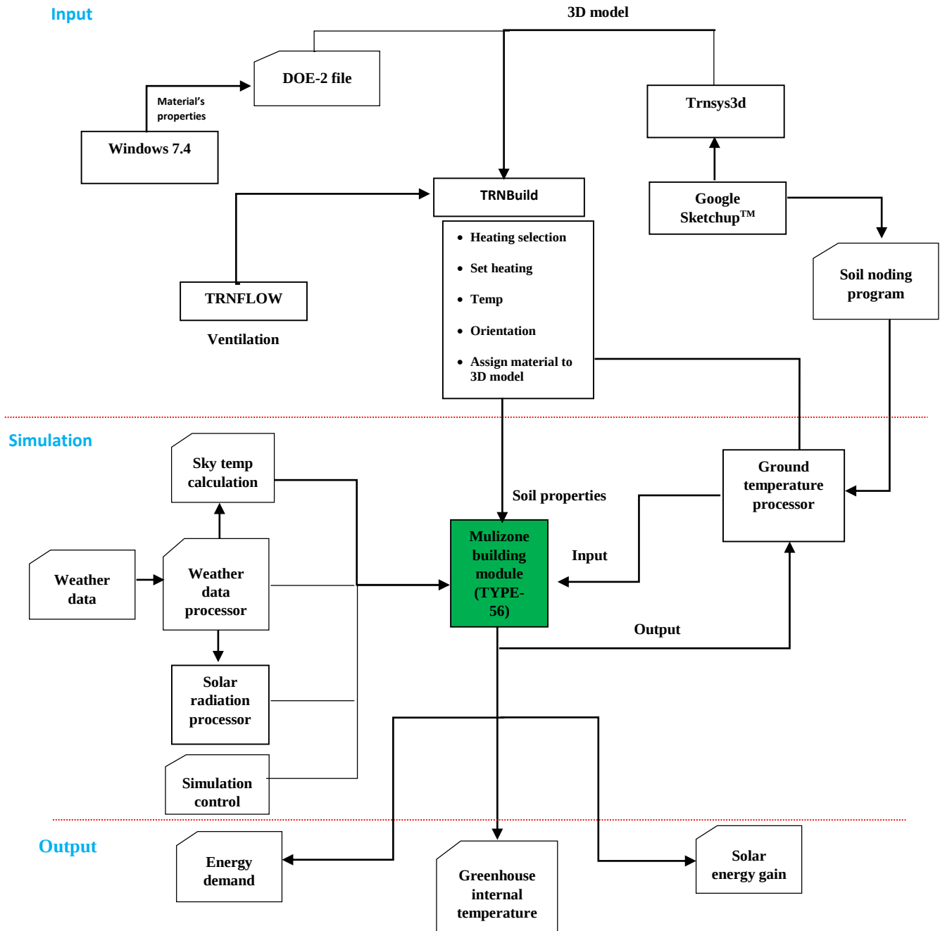
Figure 1: BES Flow chart in TRNSYS18.
