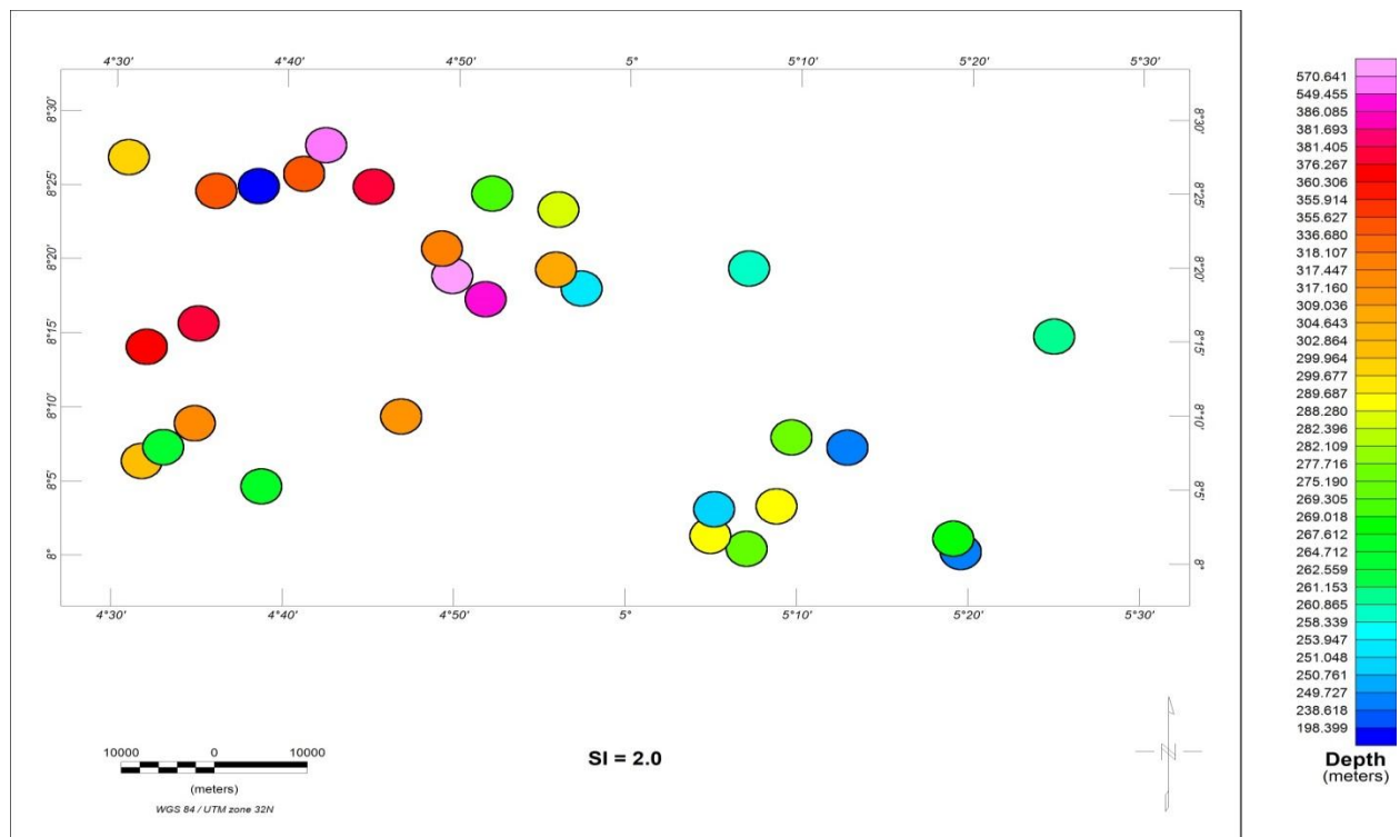
Figure 5. The Euler Deconvolution Depth Plot of the Study Area for S.I = 2.0
