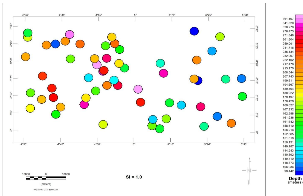
Figure 4. The Euler Deconvolution Depth Plot of the Study Area for S.I = 1.0
