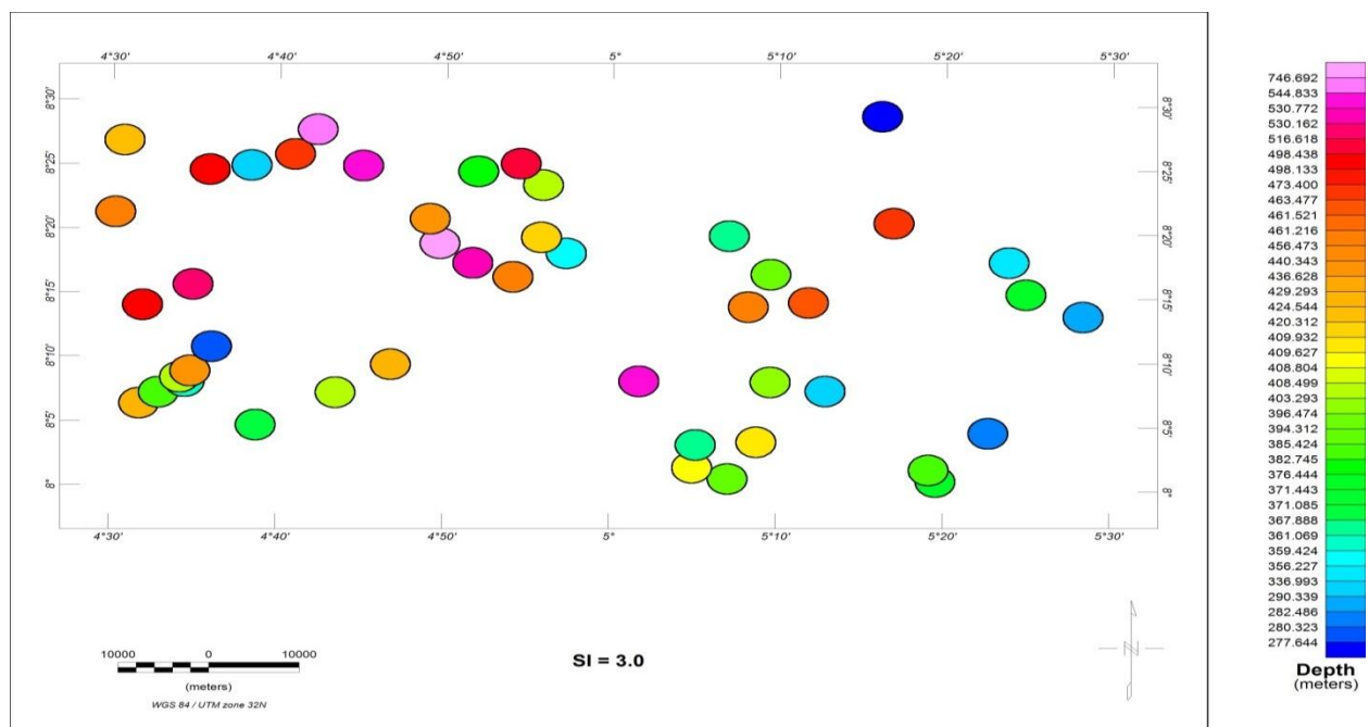
Figure 6. The Euler Deconvolution Depth Plot of the Study Area for S.I = 3.0
