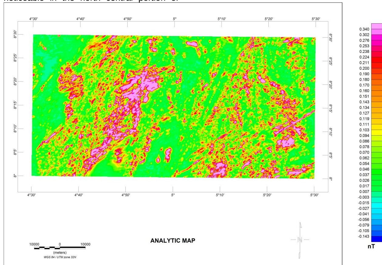
Figure 3. Analytical Signal Map of the Study Area
