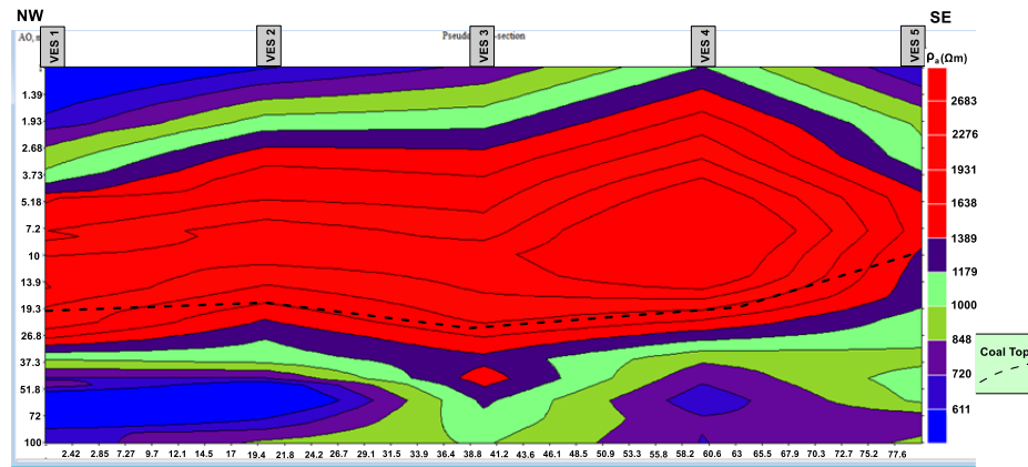
Figure 8: 2D pseudo-section along profile 1.
