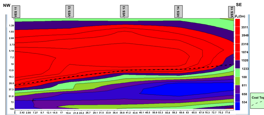
Figure 10: 2D pseudo-section along profile 3.
