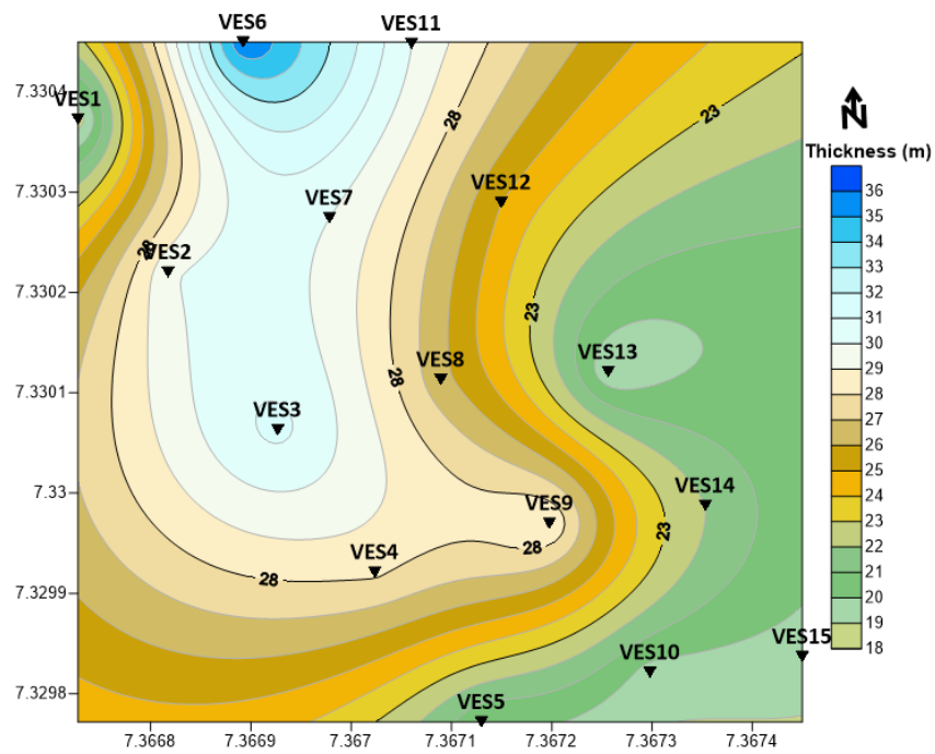
Figure 11: 2D Overburden thickness map.
