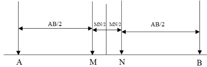
Figure 3: Schlumberger VES configuration (Kearey et al. 2002).
