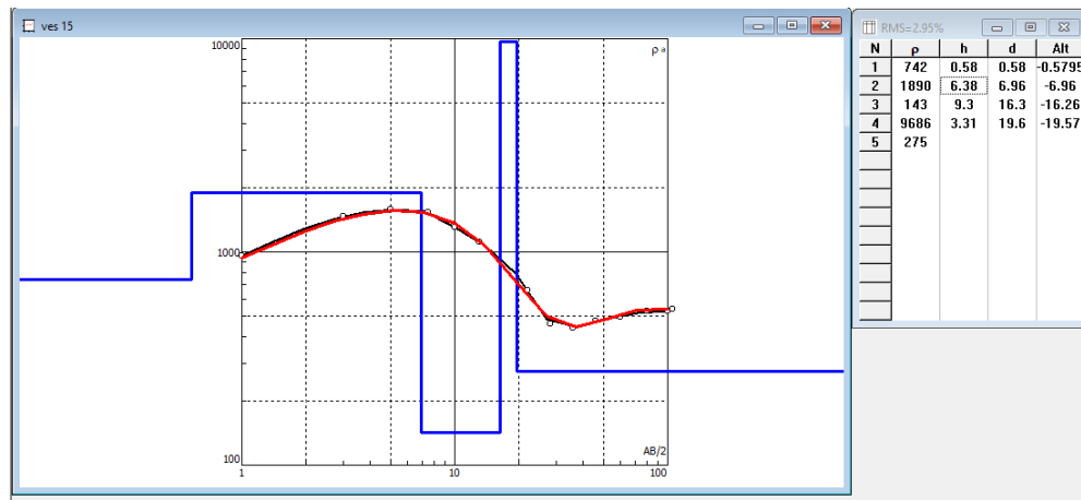
Figure 5: Typical field curve for VES 3.
