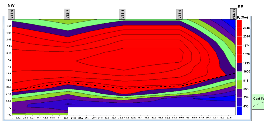
Figure 9: 2D pseudo-section along profile 2.
