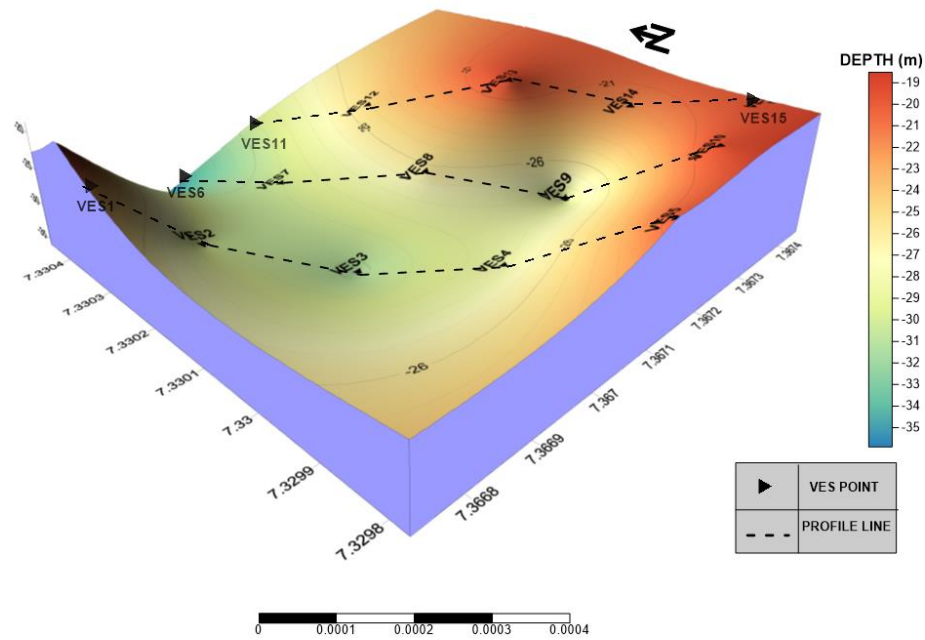
Figure 12: 3D Coal-top surface map.
