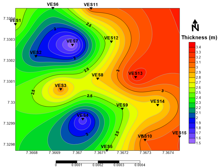
Figure 13: 2D Coal thickness map.
