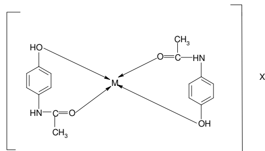
Fig II: Proposed structure for \text{M}(\text{Par})_2\text{X}_n
