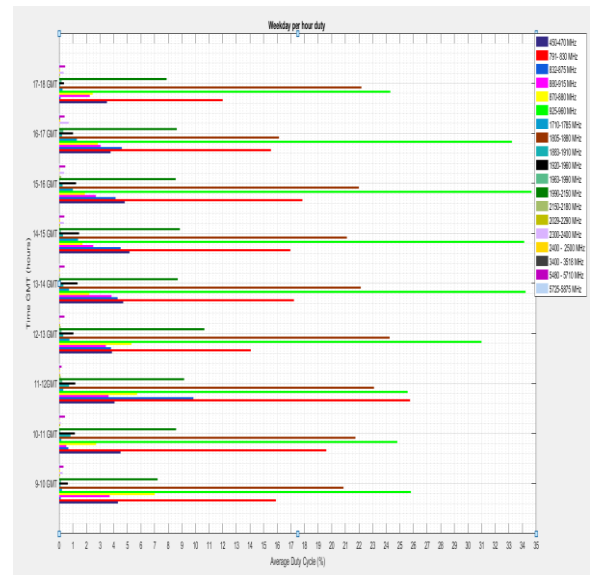
Fig. 7. An average duty cycle of each frequency band per hour
