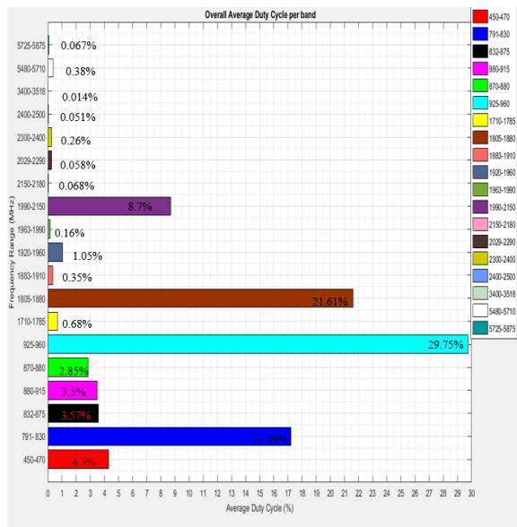
Fig. 8. Overall Average Duty Cycle per band
