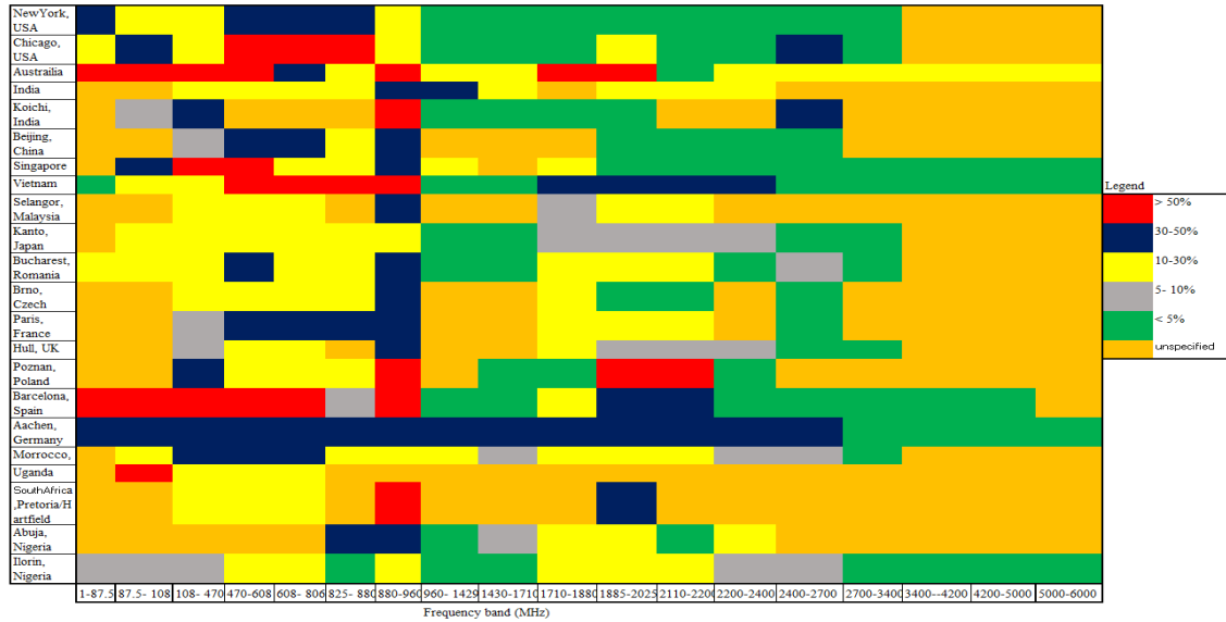
Fig. 2. Graphical representation of spectrum occupancy measurement carried out globally [6]
