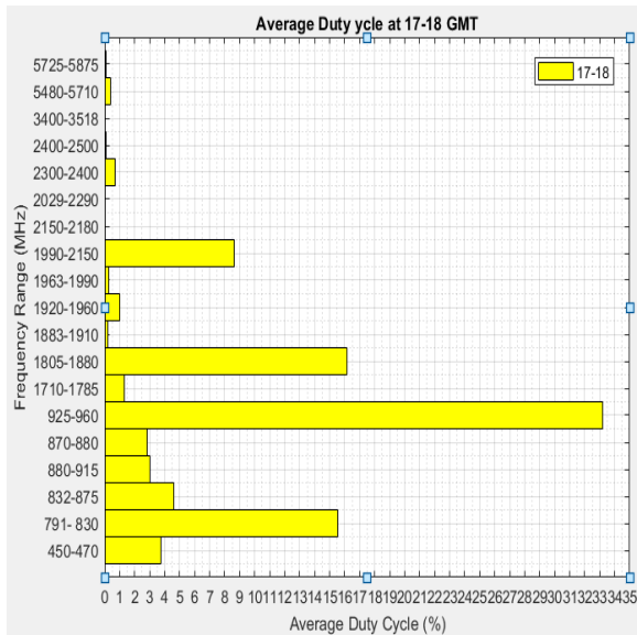
Fig. 16. Average Duty Cycle of Frequency bands between 17:00-18:00 GMT
