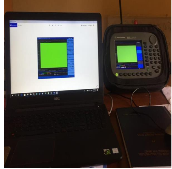
Fig. 4. Spectrum Periodogram Measurement Setup
