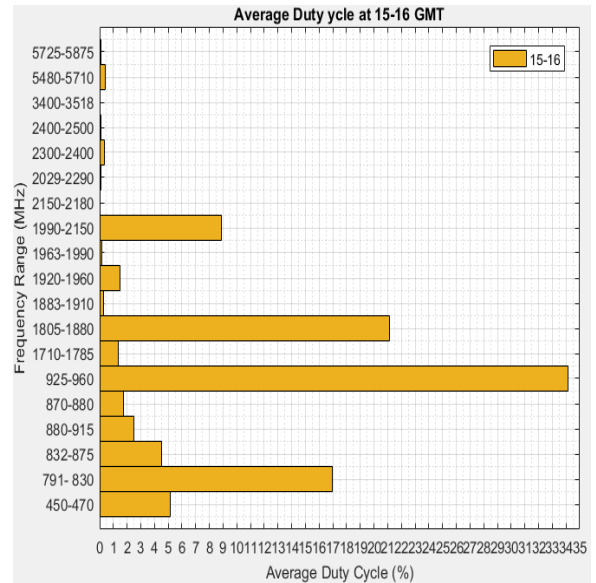
Fig. 14. Average Duty Cycle of Frequency bands between 15:00-16:00 GMT
