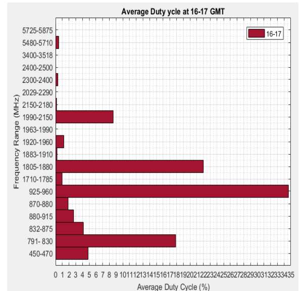
Fig. 15. Average Duty Cycle of Frequency bands between 16:00-17:00 GMT
