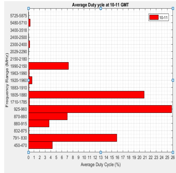
Fig. 10. Average Duty Cycle of Frequency bands between 10:00-11:00 GMT
