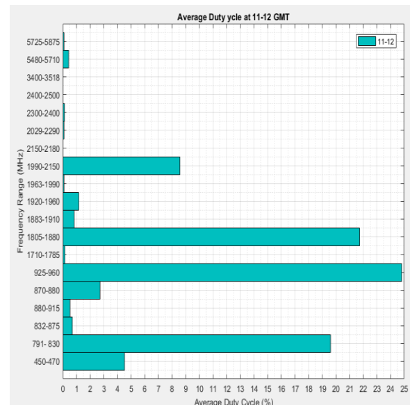
Fig. 11. Average Duty Cycle of Frequency bands between 11:00-12:00 GMT
