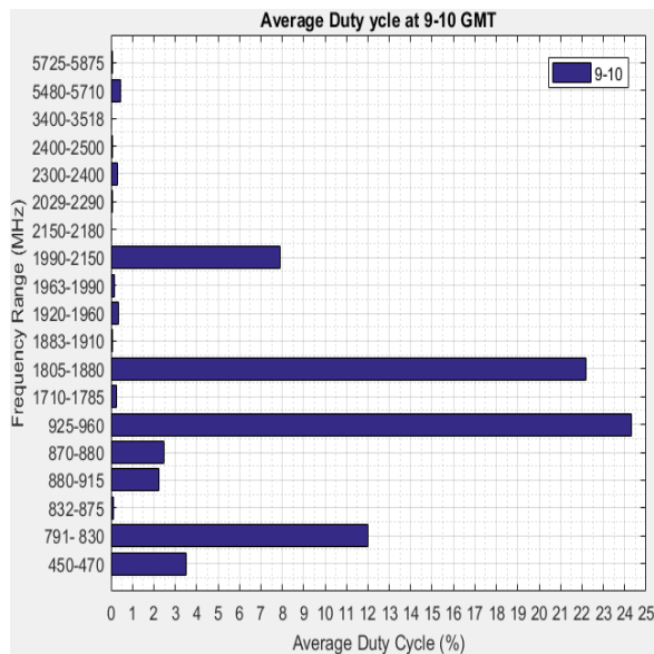
Fig. 9. Average Duty Cycle of Frequency bands between 9:00-10:00 GMT
