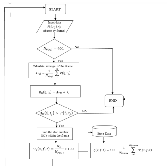
Fig. 5. Flowchart of Average Duty Cycle
