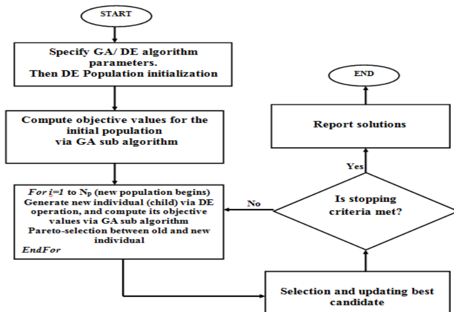
Figure 4 Flowchart of the proposed hybrid DE-GA Optimization algorithm
