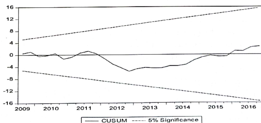
Figure 3: CUSUM tests
