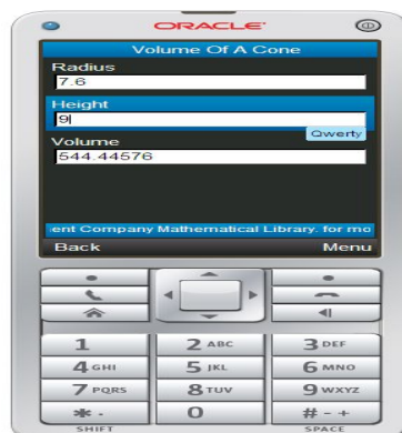
Fig. 5: The result of a volume of a cone with a radius of 7.6 and height of 9
