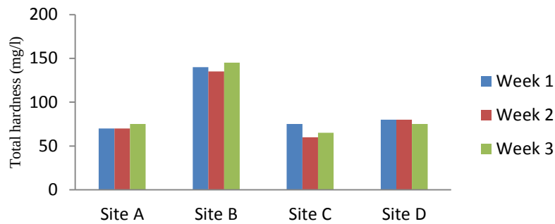
Figure 6: Average total hardness of water samples from the poultry pens (mg/l).
