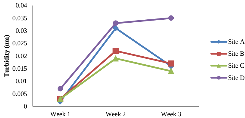
Figure 3: Average turbidity of water samples from the poultry pens
