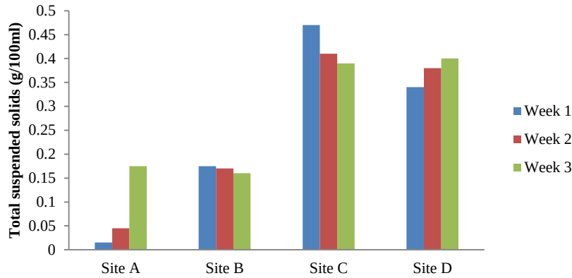
Figure 5: Average total suspended solids of water sample from the poultry pens.
