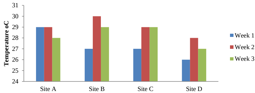
Figure 2: Average temperature of water sample from the poultry pens.
