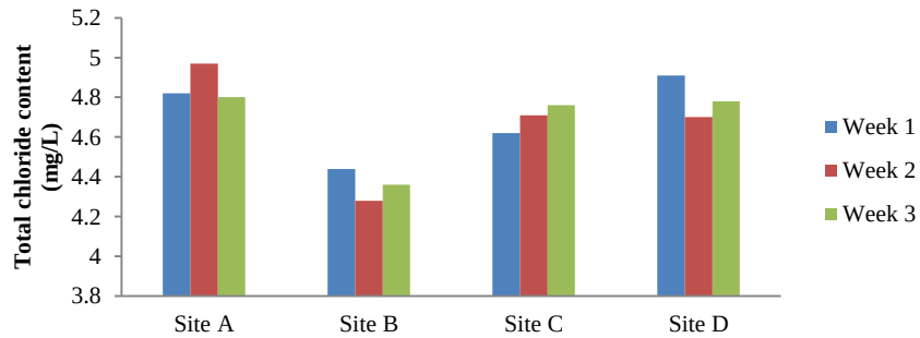
Figure 4: Average total chloride content of water sample from the poultry pens
