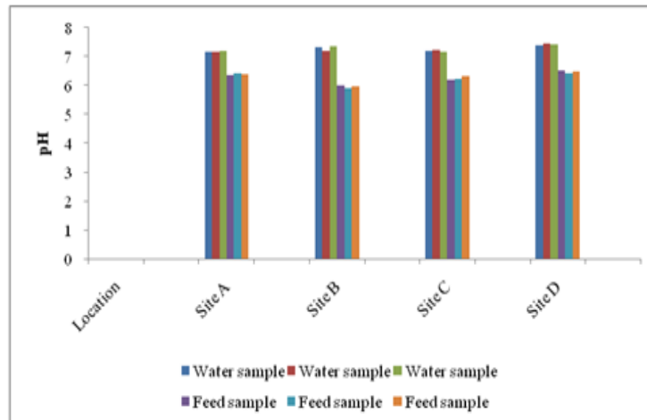
Figure 1: Average pH of water and feeds from the poultry pens
