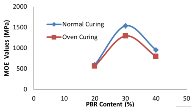
Figure 2: Effects of PBR Content on MOE Values
