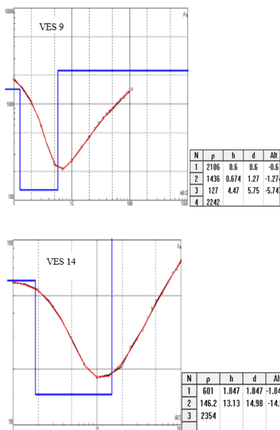
Figure 3: Resistivity curve types obtained from resistivity data in study area
