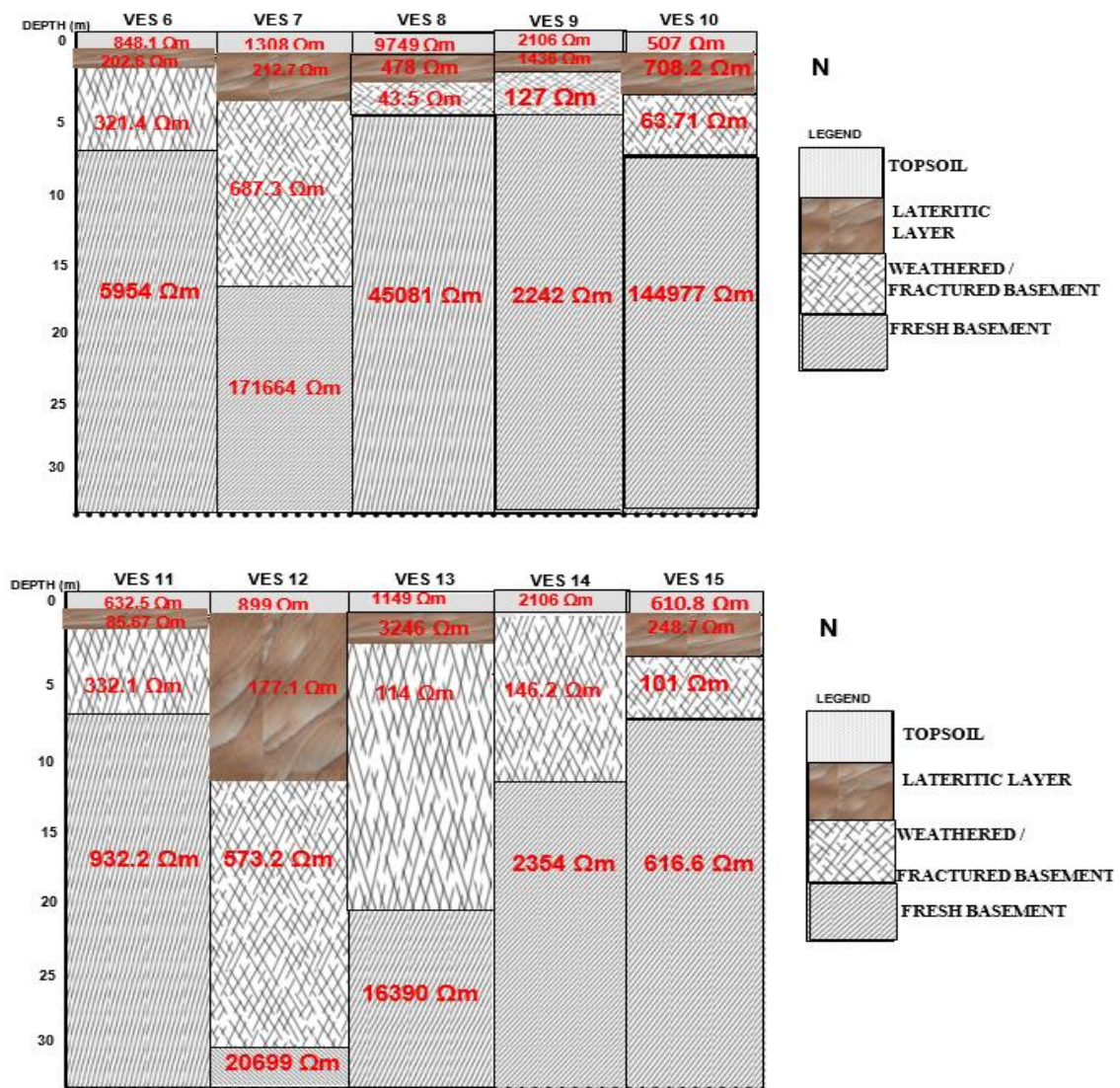
Figure 4: Geo-electric sections fromVES data in study area
