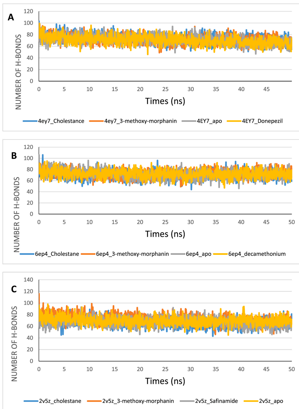
Fig. 15. The changes in the number of H-bonds during the MDS trajectory of unbound and enzyme-ligand complexes (a) human acetylcholinesterase (hAChE) (b) human butyrylcholinesterase (hBChE) (c) human Monoamine oxidase (MAO-B).
