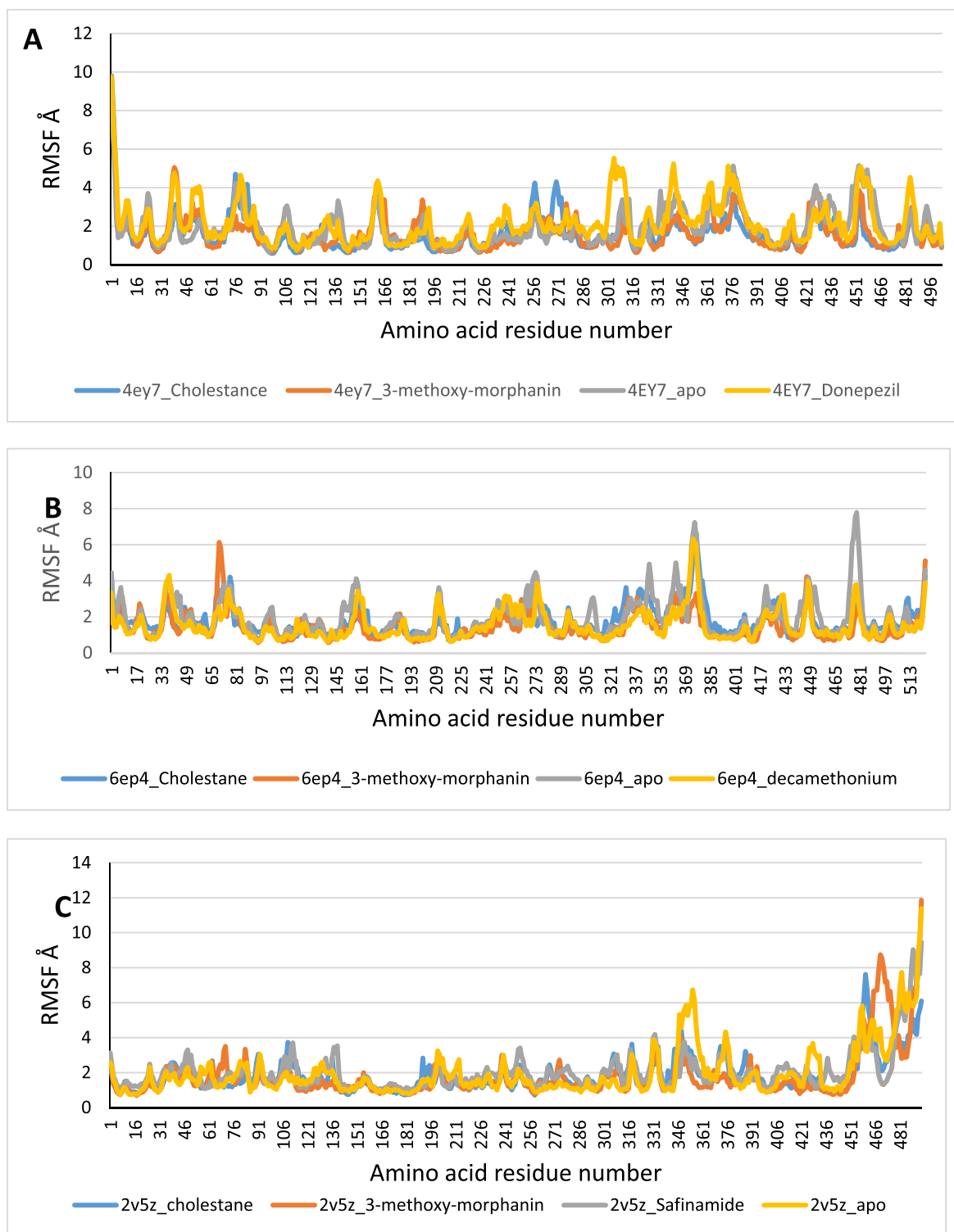
Fig. 12. Per residue RMSF plots of molecular dynamics (MD) simulation of unbound and enzyme-ligand complexes to (a) human acetylcholinesterase (hAChE) (b) human butyrylcholinesterase (hBChE) (c) human Monoamine oxidase (MAO-B).
