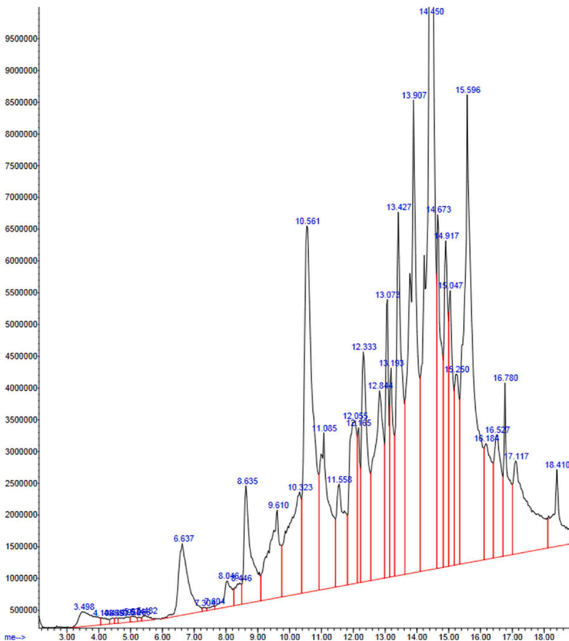
Fig. 4. Chromatogram of phytocompounds in n-hexane fraction of methanol O. gratissimum .
