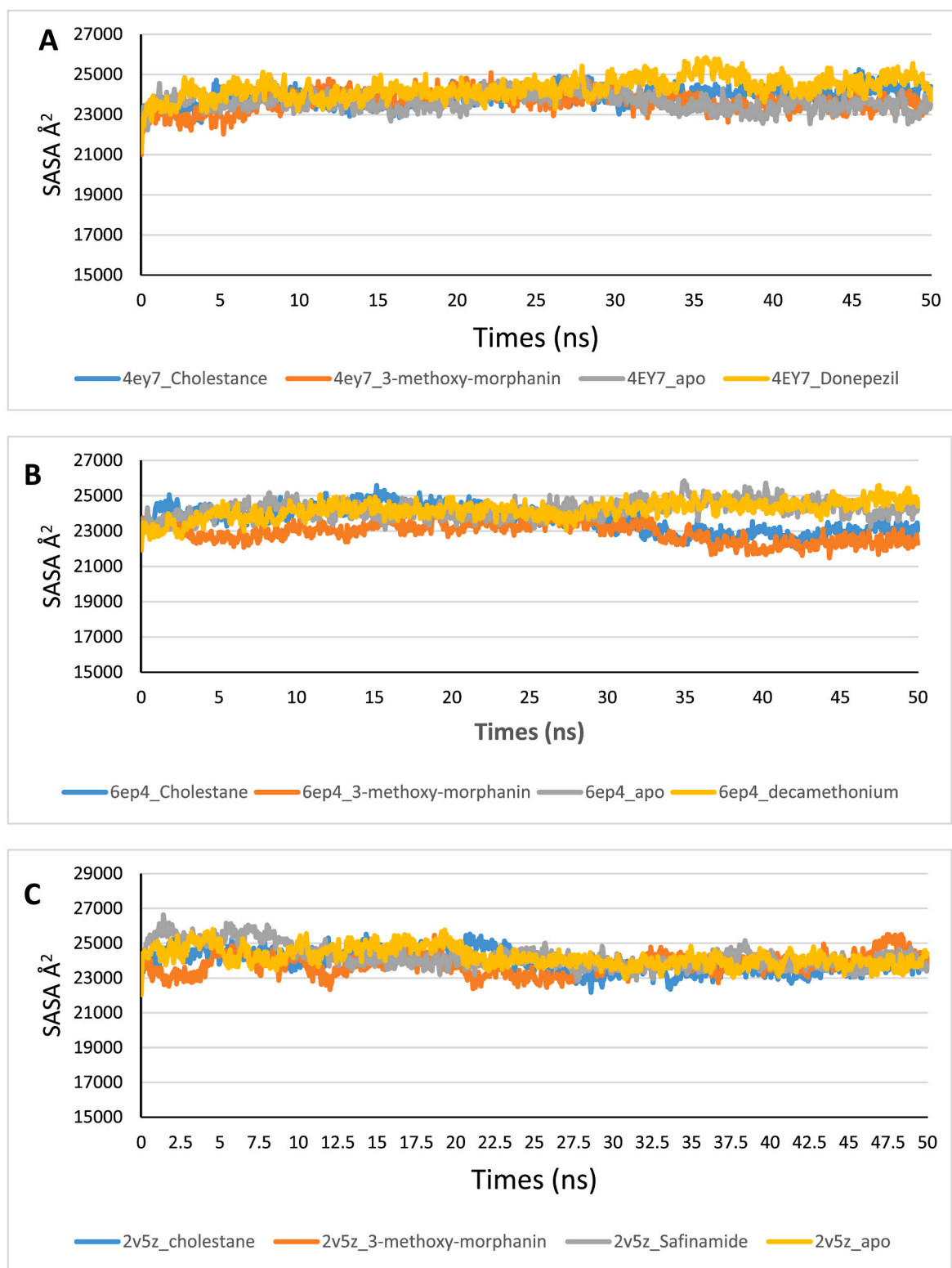
Fig. 14. The SASA plots of molecular dynamics (MD) simulation of unbound and enzyme-ligand complexes (a) human acetylcholinesterase (hAChE) (b) human butyrylcholinesterase (hBChE) (c) human Monoamine oxidase (MAO-B).
