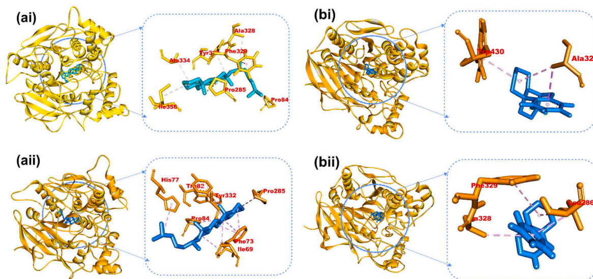
Fig. 18. Amino acid interaction of lead phytochemicals: (a) 3-methoxy-morphanin (b) cholestane in the first cluster (i) and last cluster (ii) of hBChE complexes obtained from the cluster analysis of the MDS trajectories.
