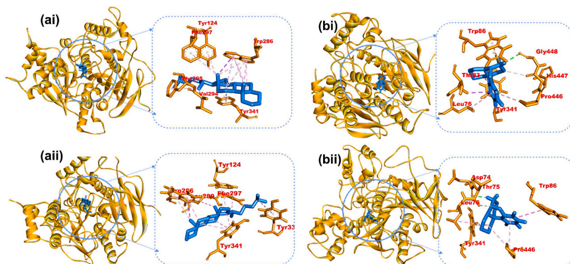
Fig. 17. Amino acid interaction of lead phytochemicals: (a) 3-methoxy-morphanin (b) cholestane in the first cluster (i) and last cluster (ii) of hAChE complexes obtained from the cluster analysis of the MDS trajectories.
