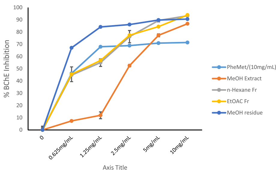
Fig. 2. BChE inhibitory activity of the methanol extract and solvent-solvent partition fractions of O. gratissimum leaves. Data are expressed as mean \pm SD ( n = 2 ). MeOH—methanol extract; EtOAc—ethylacetate fraction; Res MeOH—residual fraction after partitioning with n-hexane and ethylacetate.
