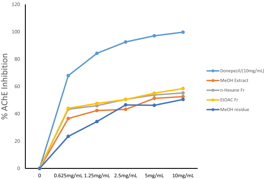
Fig. 1. AChE inhibitory activity of the methanol extract and solvent-solvent partition fractions of O. gratissimum leaves. Data are expressed as mean \pm SD ( n = 2 ). MeOH—methanol extract; EtOAc—ethylacetate fraction; Res MeOH—residual fraction after partitioning with n-hexane and ethylacetate.
