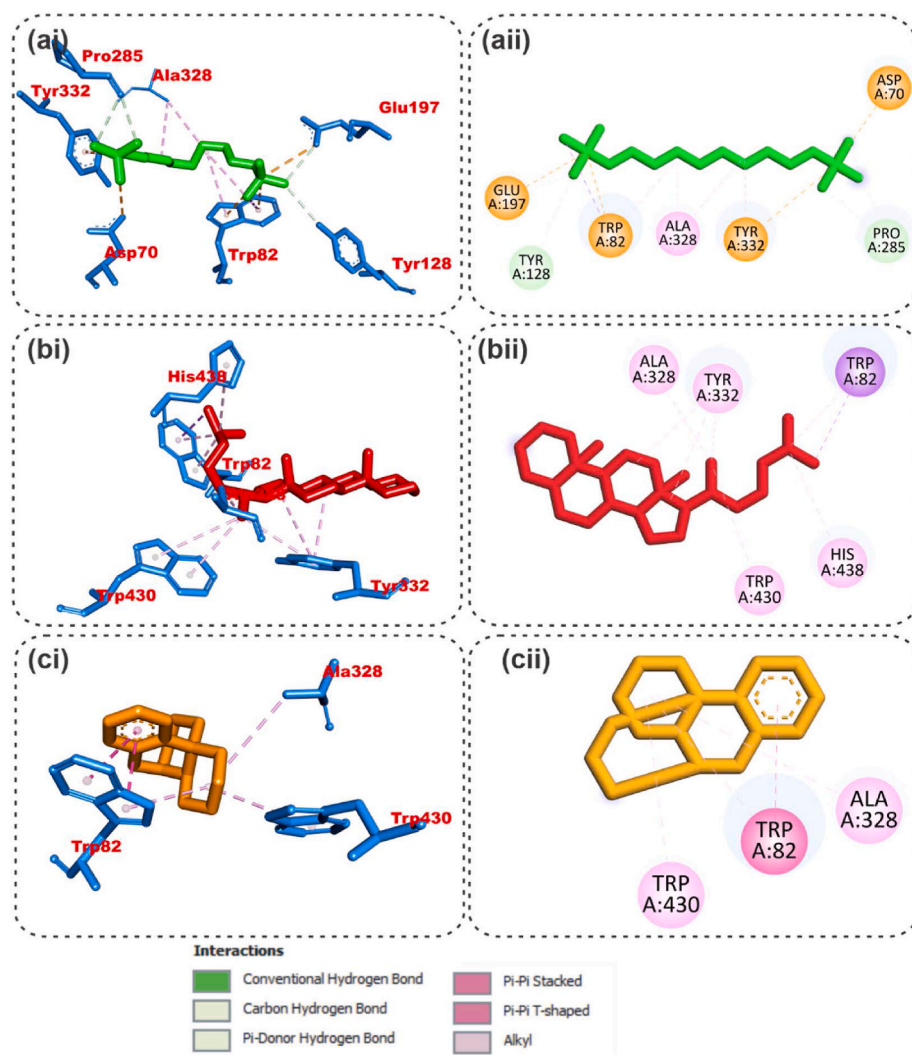
Fig. 8. Amino acid interactions of lead phytochemicals and reference inhibitor from the docking analysis of GC-MS identified compounds from Ocimum gratissimum in the active site groove of human butyrylcholinesterase. The ligands are presented in stick representations and differentiated by colours (a) Green: decamethonium (reference inhibitor) (b) Red: cholestane (c) gold: 3-methoxy-morphanin. (For interpretation of the references to colour in this figure legend, the reader is referred to the Web version of this article.)
