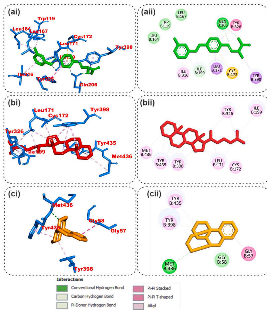
Fig. 9. Amino acid interactions of lead phytochemicals and reference inhibitor from the docking analysis of GC-MS identified compounds from Ocimum gratissimum in the active site of human mono amine oxidase . The ligands are presented in stick representations and differentiated by colours (a) Green: Safinamide (reference inhibitor) (b) Red: Cholestane (c) gold: 3-methoxy-morphanin. (For interpretation of the references to colour in this figure legend, the reader is referred to the Web version of this article.)
