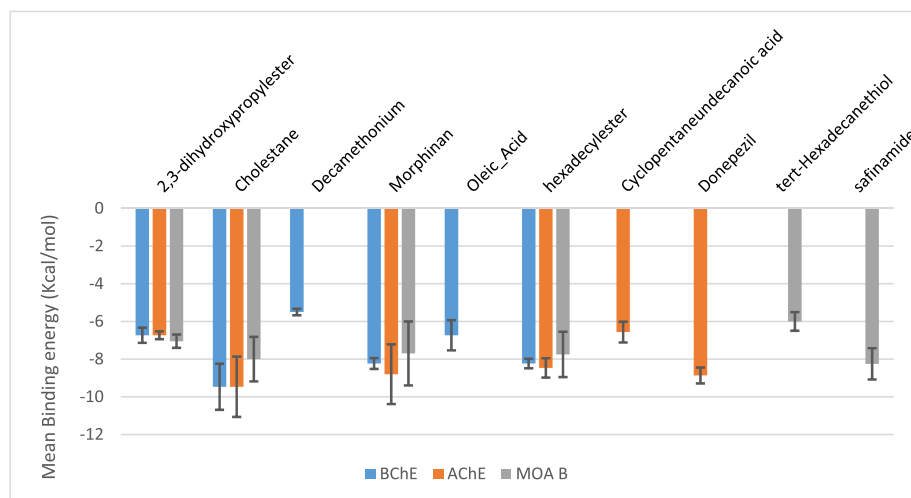
Fig. 16. The average binding energies of the reference inhibitors and five lead phytochemicals against representative conformation gotten from the clustering analysis of the MD simulation trajectories of AChE, BChE and MAO-B enzyme. Number of clusters: AChE (4), BChE (4) and MAO-B (6) enzyme.
