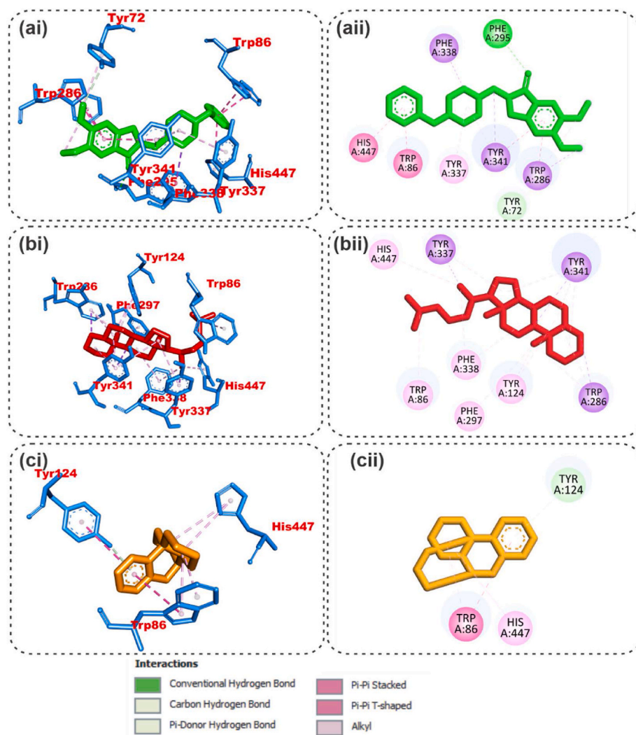
Fig. 7. Amino acid interactions of lead phytochemicals and reference inhibitor from the docking analysis of GC-MS identified compounds from Ocimum gratissimum in the active site groove of human butyrylcholinesterase. The ligands are presented in stick representations and differentiated by colours (a) Green: donepezil (reference inhibitor) (b) Red: cholestane (c) gold: 3-methoxy-morphanin. (For interpretation of the references to colour in this figure legend, the reader is referred to the Web version of this article.)
