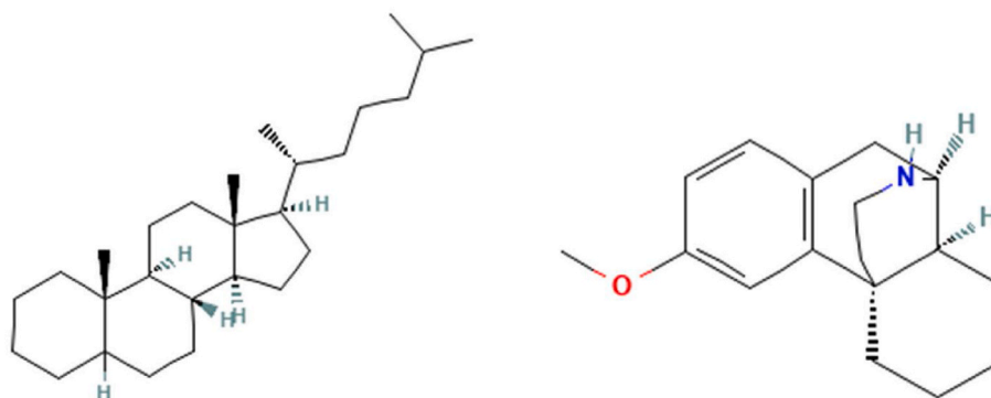
Fig. 6. Chemical structure of lead phytochemicals (a) Cholestane (b) 3-Methoxy-morphanin.
