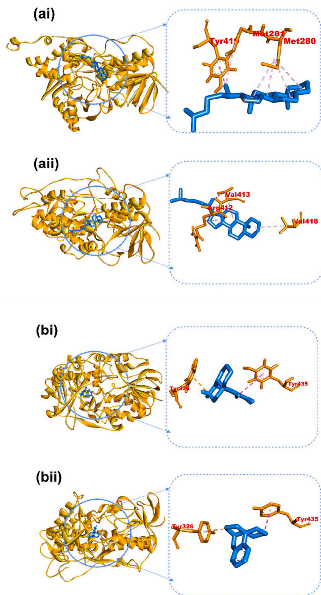
Fig. 19. Amino acid interaction of lead phytochemicals: (a) 3-methoxy-morphanin (b) cholestane in the first cluster (i) and last cluster (ii) of MAO-B complexes obtained from the cluster analysis of the MDS trajectories.
