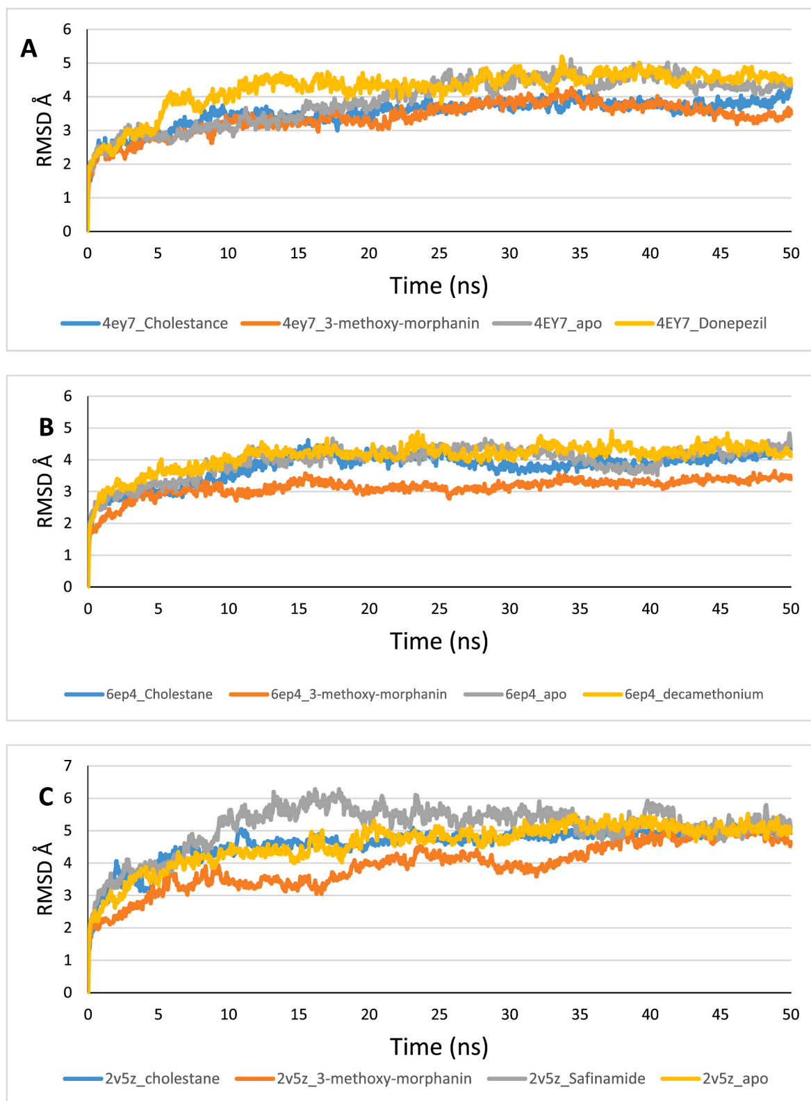
Fig. 11. The Backbone-RMSD plots of molecular dynamics (MD) simulation of unbound and enzyme-ligand complexed to (a) human acetylcholinesterase (hAChE) (b) human butyrylcholinesterase (hBChE) (c) human Monoamine oxidase (MAO-B).
