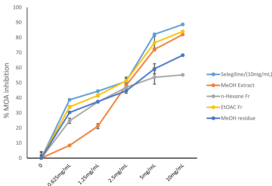
Fig. 3. Monoamine oxidase inhibitory activity of the methanol extract and solvent-solvent partition fractions of O. gratissimum leaves. Data are expressed as mean \pm SD ( n = 2 ). MeOH—methanol extract; EtOAc—ethylacetate fraction; Res MeOH—residual fraction after partitioning with n-hexane and ethylacetate.
