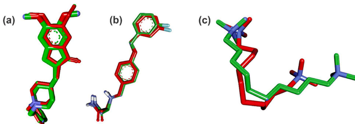
Fig. 5. Superimposition of docked conformer of the native ligand on the extracted conformation of (a) donepezil, (b) safinamide and (c) decamethonium. Red: selected docked conformer and Green: extracted native ligand conformer. (For interpretation of the references to colour in this figure legend, the reader is referred to the Web version of this article.)
