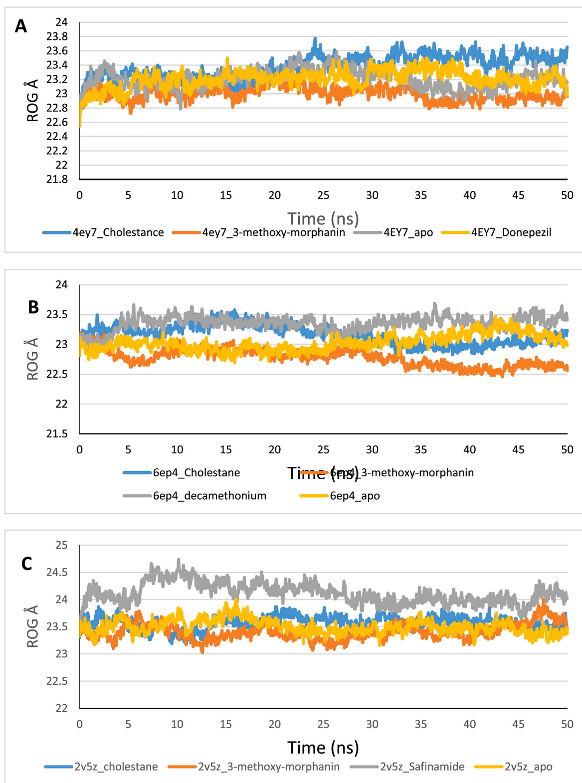
Fig. 13. The RoG plots of molecular dynamics (MD) simulation of unbound and enzyme-ligand complexes (a) human acetylcholinesterase (hAChE) (b) human butyrylcholinesterase (hBChE) (c) human Monoamine oxidase (MAO-B).
