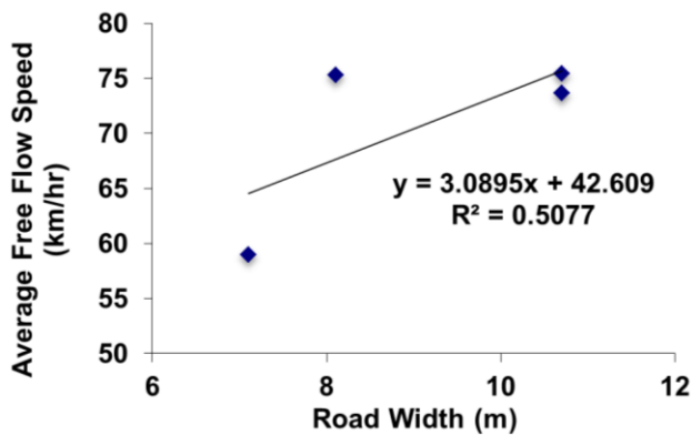
Figure 6: Average free flow speed against road width
